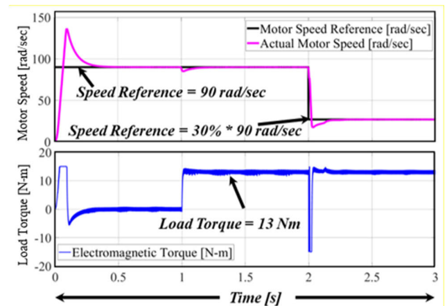
FIGURE 7. Tracking the performance of five-phase induction motor from 100% to 20% of rated speed at rated torque.
