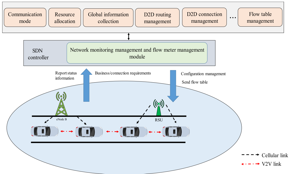
FIGURE 2. Proposed system model of V2X-SDN.
