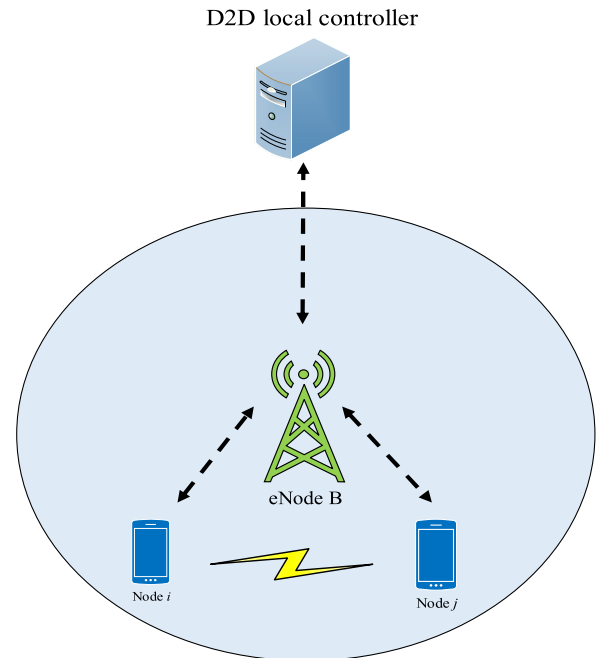
FIGURE 5. Position measurement between nodes for single-hop D2D communication.
