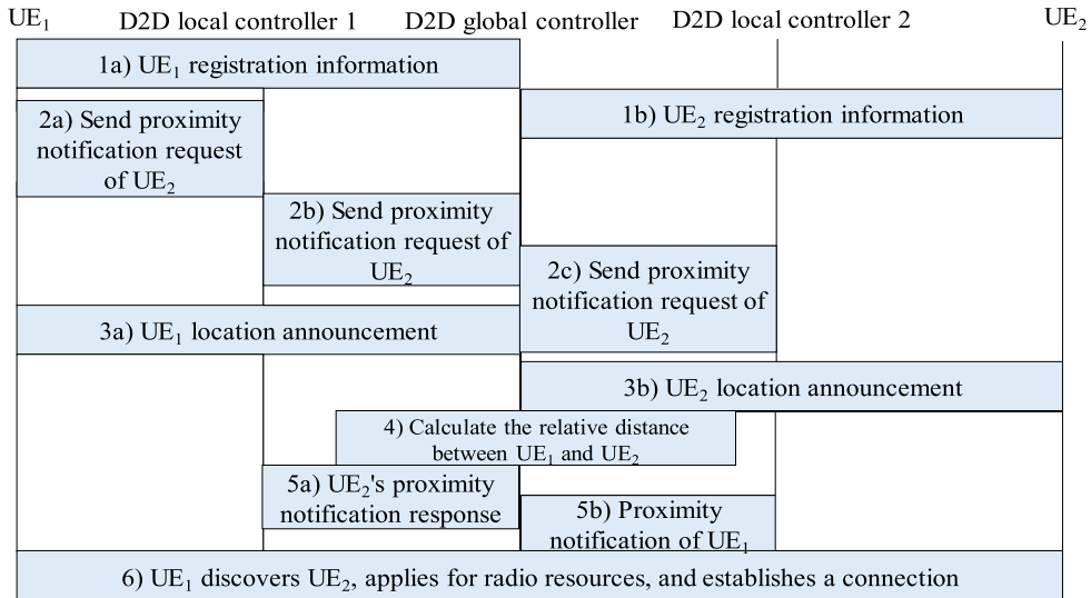
FIGURE 7. D2D global neighbor discovery signaling process.
