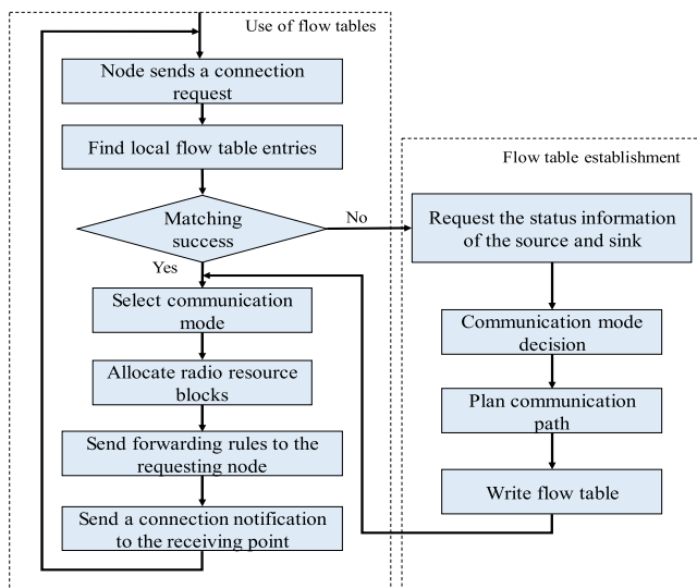
FIGURE 9. Flowchart for management of flow table.
