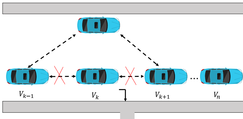
FIGURE 11. V2V path restoration example.
