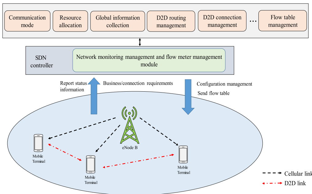
FIGURE 1. Proposed system model of D2D-SDN.
