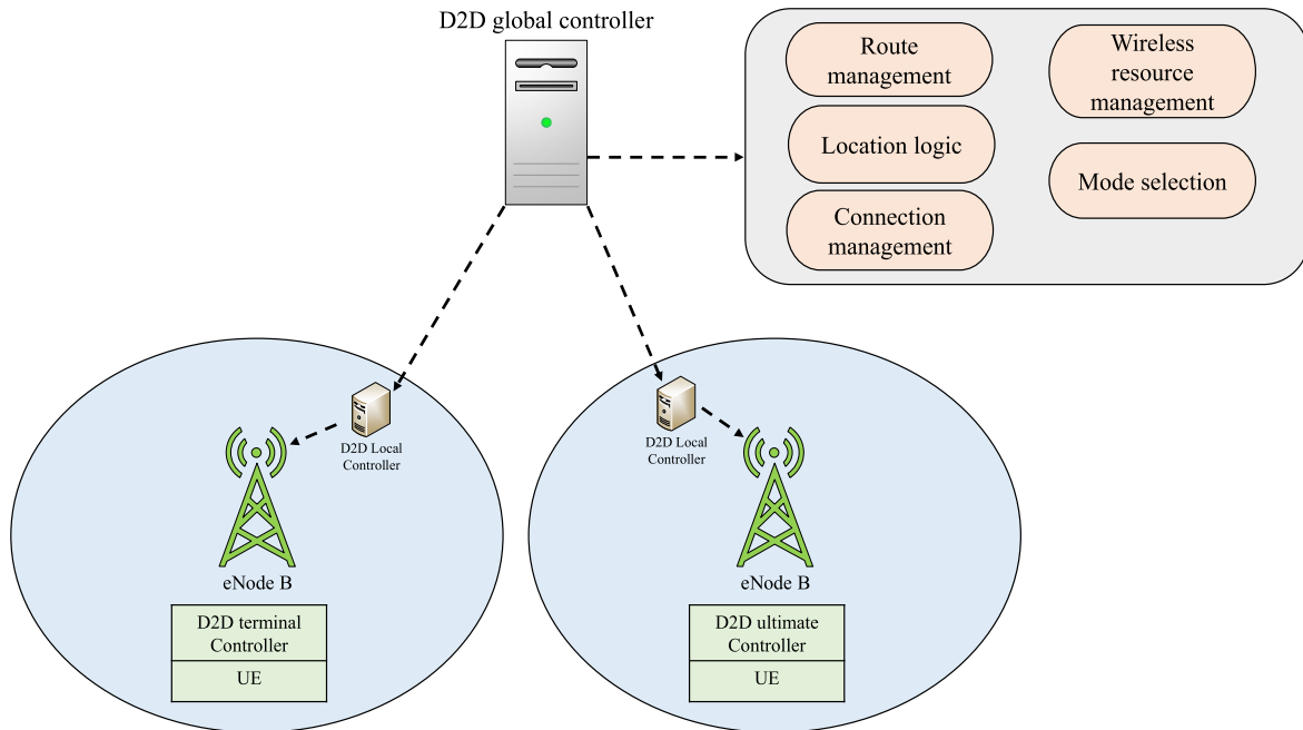
FIGURE 3. Layered architecture for D2D-SDN communication.
