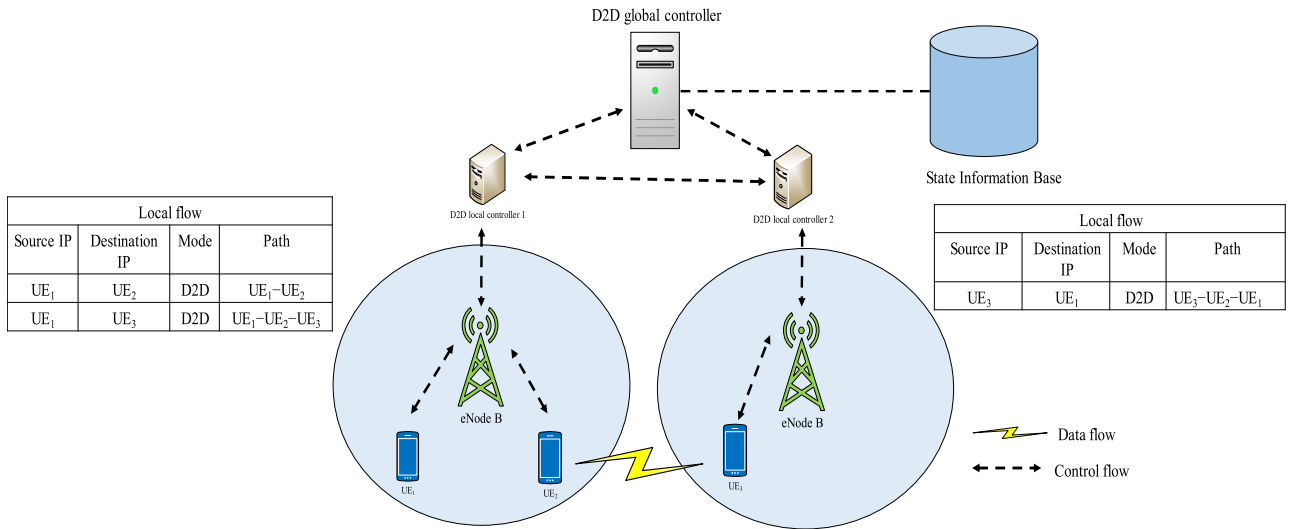
FIGURE 8. Route management within/between base stations.
