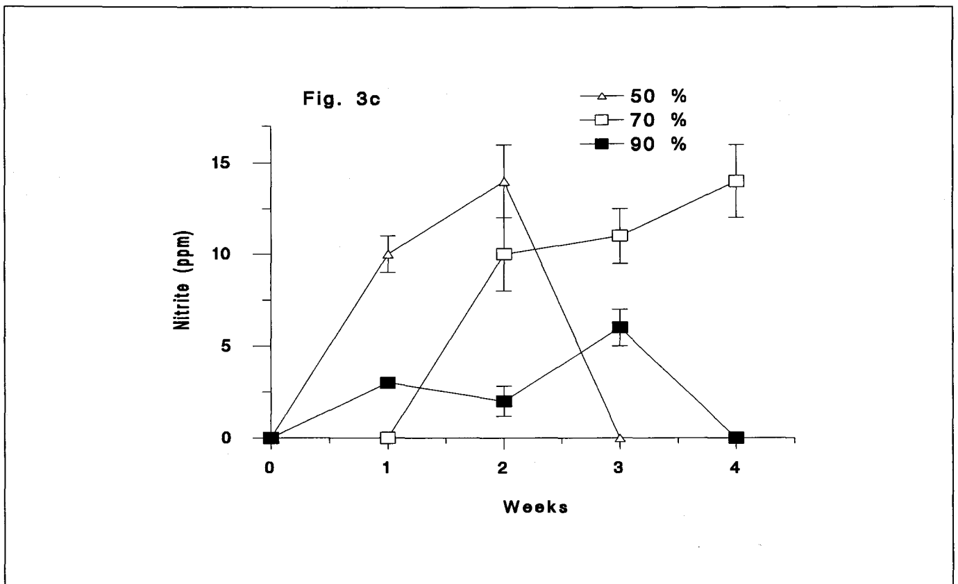
Fig 3c. Effect of moisture content on nitrite concentration in soil samples treated with (\text{NH}_4)_2\text{SO}_4 at 5 mg/g. All values are means of triplicates \pm S.D.
