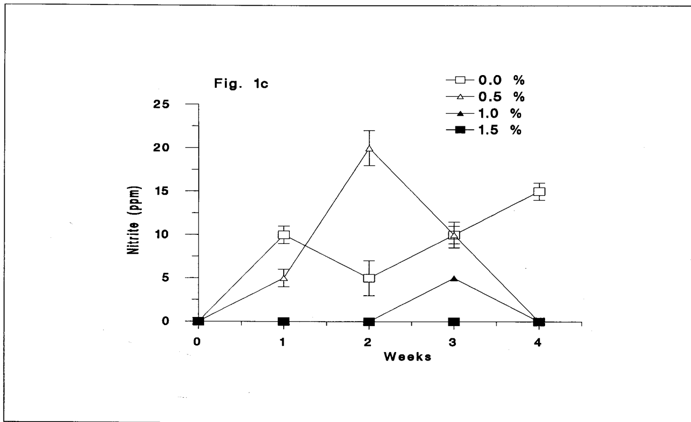
Fig 1c. Effect of salinity on nitrite concentration in soil samples treated with (\text{NH}_4)_2\text{SO}_4 at 5 mg/g. All values are means of triplicates \pm S.D.
