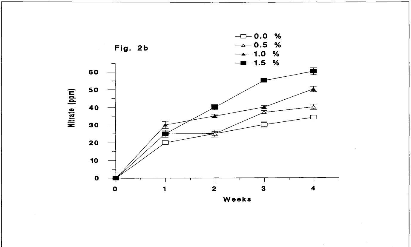
Fig 2b. Effect of organic matter on nitrate concentration in soil samples treated with (\text{NH}_4)_2\text{SO}_4 at 5 mg/g. All values are means of triplicates \pm S.D.
