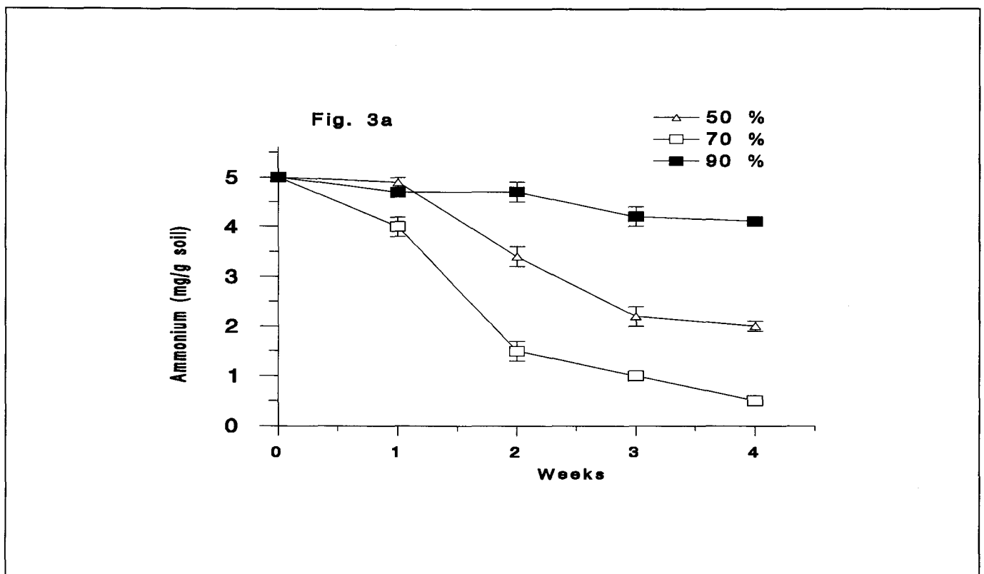
Fig 3a. Effect of moisture content on ammonium concentration in soil samples treated with (\text{NH}_4)_2\text{SO}_4 at 5 mg/g. All values are means of triplicates \pm S.D.
