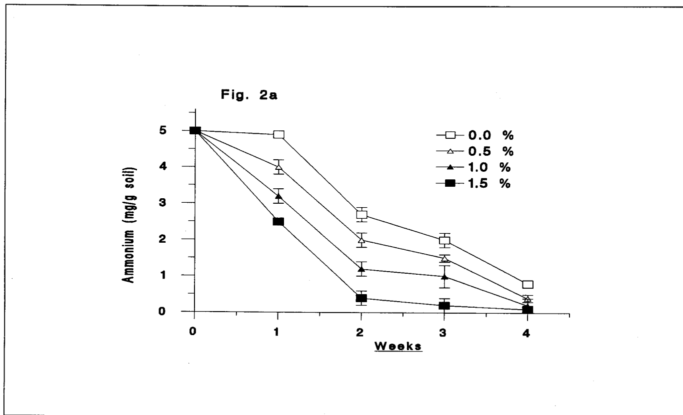
Fig 2a. Effect of organic matter on ammonium concentration in soil samples treated with (\text{NH}_4)_2\text{SO}_4 at 5 mg/g. All values are means of triplicates \pm S.D.
