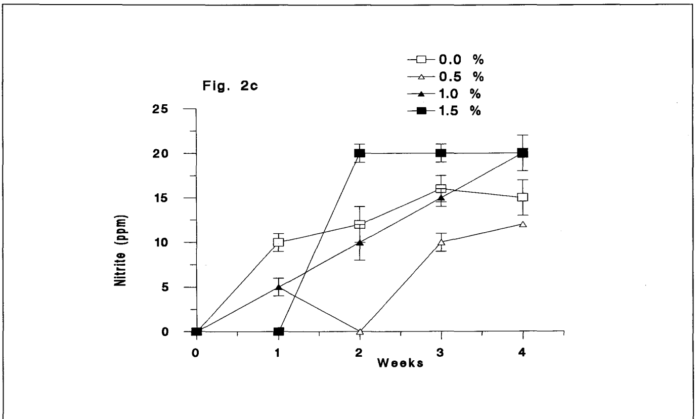
Fig 2c. Effect of organic matter on nitrite concentration in soil samples treated with (\text{NH}_4)_2\text{SO}_4 at 5 mg/g. All values are means of triplicates \pm S.D.
