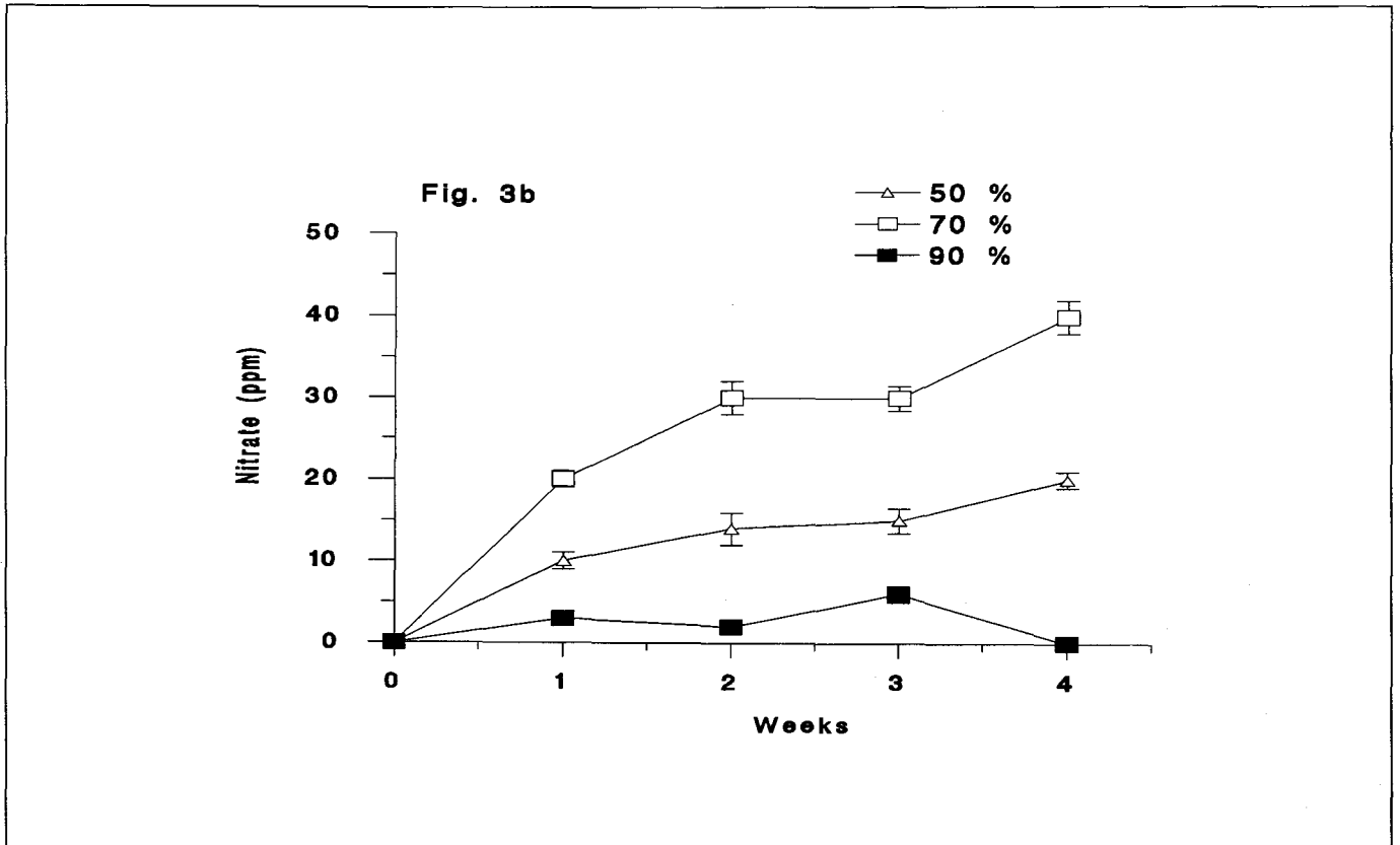
Fig 3b. Effect of moisture content on nitrate concentration in soil samples treated with (\text{NH}_4)_2\text{SO}_4 at 5 mg/g. All values are means of triplicates \pm S.D.
