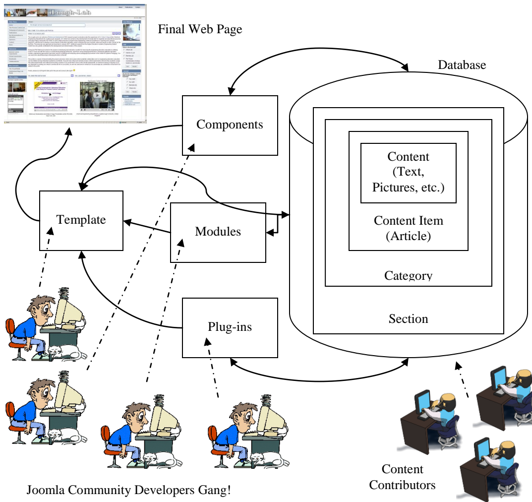
Figure 8. General architecture of the Joomla WCMS
