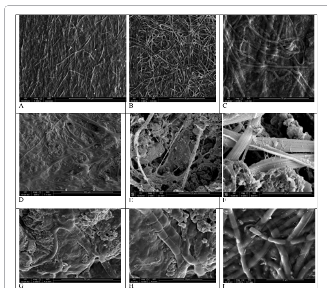
Figure 3: Environmental scanning electron microscopy images showing: cyanobacterial filaments within the pond water samples (A, B, C) and microbial mat, cyanobacterial filaments and diatoms (D, E, F) with extracellular polymeric substances (EPS). Precipitation of minerals (mainly halite and calcite) on EPS (G, H). Thick biofilm from pond water binding and trapping bacterial cells (I). Cyanobacterial filaments all embedded in a massive biofilm.
