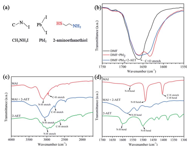
Fig. 1 Chemical structures (a) of MAI, PbI 2 and 2-AET; FTIR spectra of pure DMF, PbI 2 DMF solution and 2-AET/PbI 2 DMF solution in the range of 1750–1550 cm -1 (b); FTIR spectra of MAI, 2-AET and MAI·2-AET solid complexes in the range of 4000–1700 cm -1 (c) and 1700–1300 cm -1 (d).
