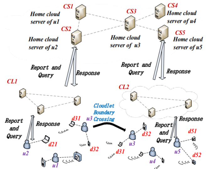
FIGURE 9. The IoT-HiTrust architecture [117].
