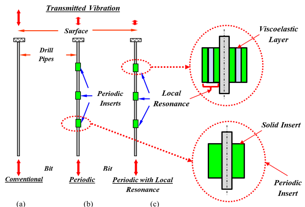
Figure 1. Schematic drawings of conventional (a), periodic (b), and periodic with local resonant inserts (c) drill-strings.
