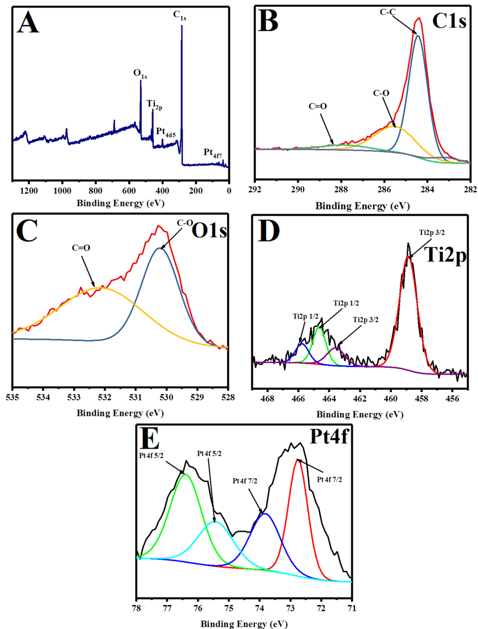
Figure 1. (A) XPS spectra survey for the synthesized hybrid graphene-Pt/TiO 2 nanostructure (B) C 1s spectra (C) O 1s spectra (D) Ti 2p spectra and (E) Pt 4f spectra for the synthesized hybrid graphene-Pt/TiO 2 nanostructure.
