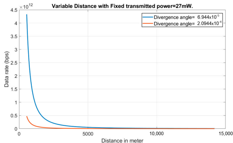
Figure 13. Data rate versus distance for two values of the divergence angle.
