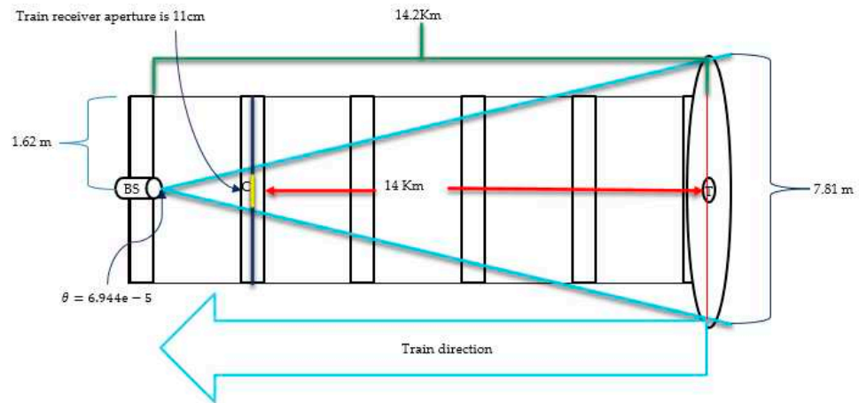
Figure 2. Top geometrical view for the proposed model (ideal case).
