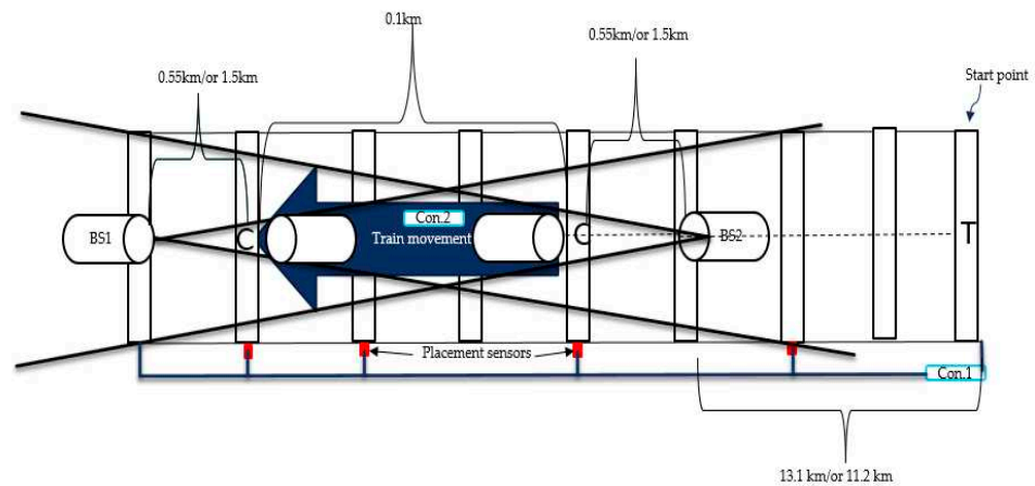
Figure 5. Overview of the handover mechanism.
