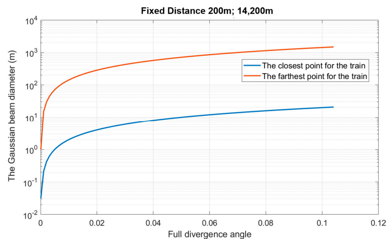
Figure 7. Gaussian beam diameter versus divergence angles for the proposed method.
