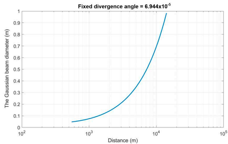
Figure 8. Gaussian beam diameter versus distance for a fixed divergence angle.
