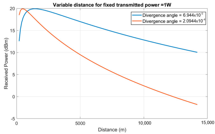
Figure 12. Received power versus distance for two values of the divergence angle (assuming a transmit power P_{tx} = 1 W).
