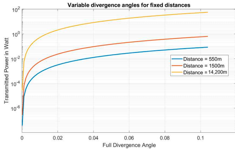
Figure 9. Transmit power versus divergence angle for several fixed distances: (a) distance of 550 m, (b) distance of 1500 m, (c) distance of 14,200 m.
