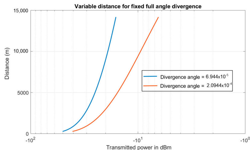
Figure 10. Distance versus transmitted power required for fixed data rate 1.25 Gbps.
