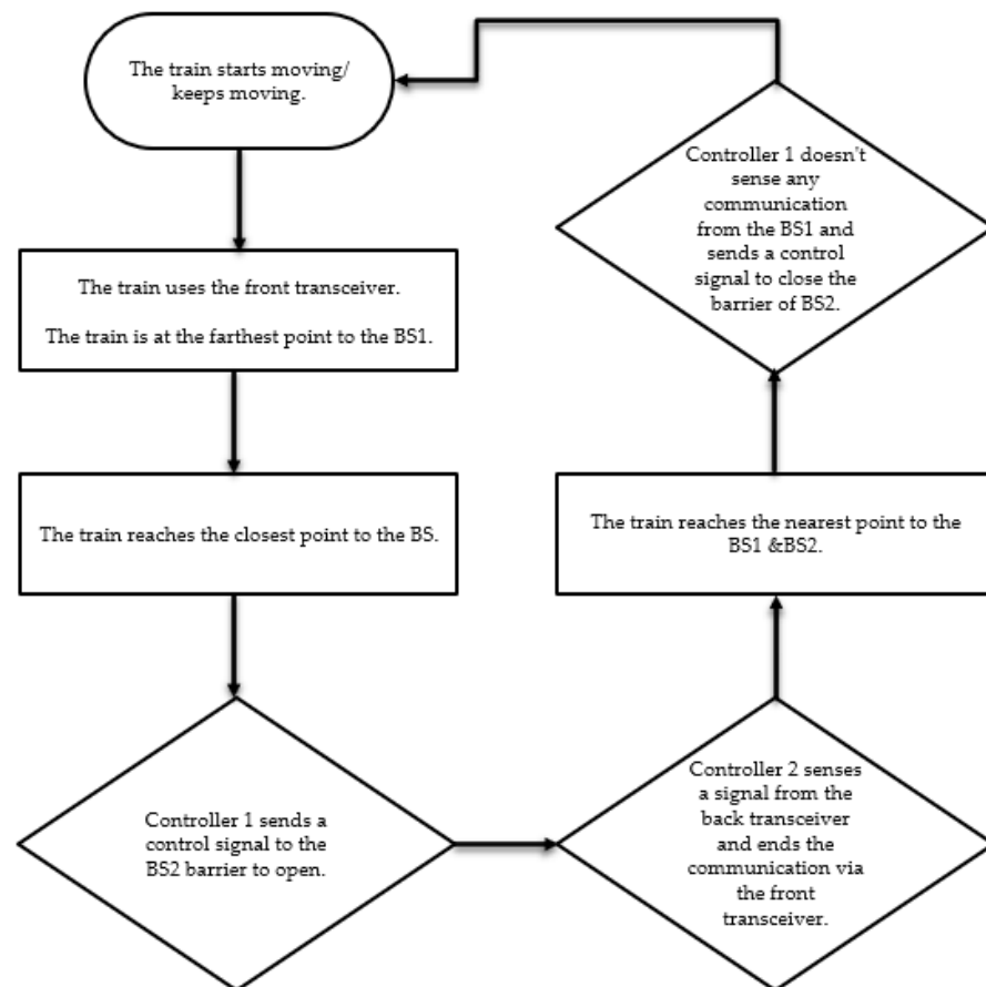
Figure 6. Flow chart of the handover process.
