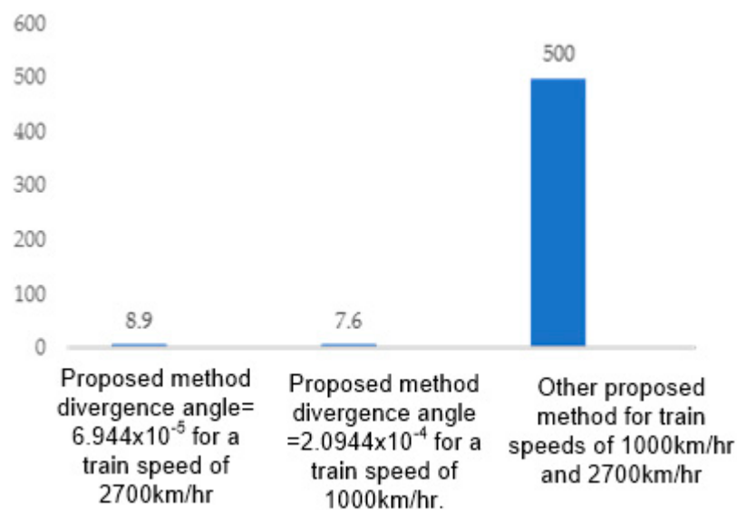
Figure 15. The number of base stations required for 100 km.
