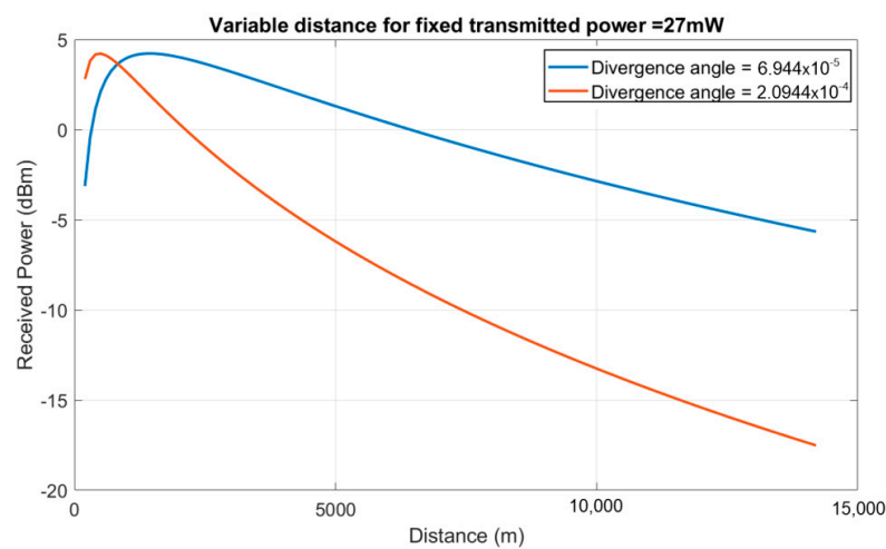
Figure 11. Received power versus variable distance for two divergence angles (assuming a transmit power P_{tx} = 27 mW).
