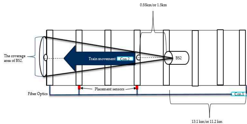
Figure 4. BS2 handover mechanism.
