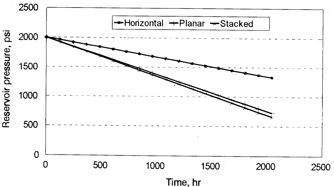
Fig. 7. Reservoir pressure decline with time.
