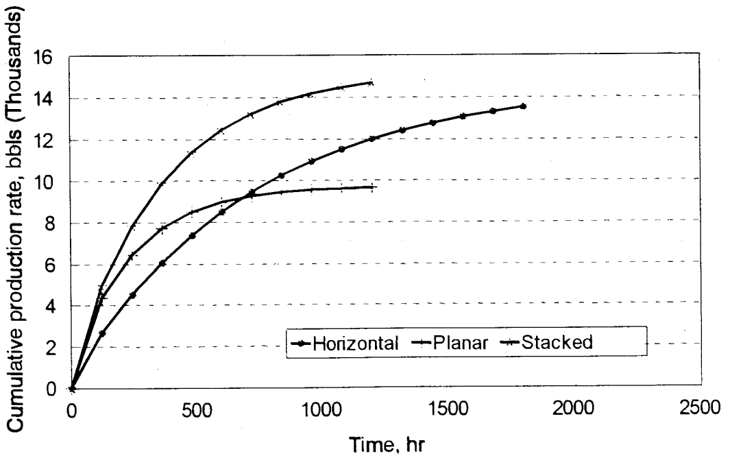
Fig. 9. Cumulative production with time.
