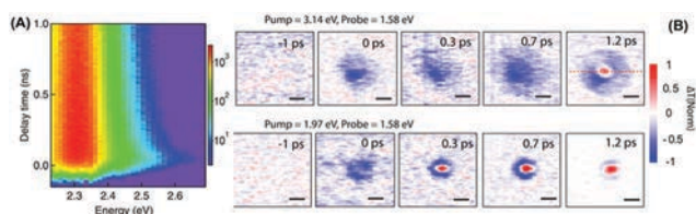
Fig. 9 (A) Hot emission observed in TRPL in single-crystal \text{MAPbBr}_3 microplates with a 100 ps lifetime. (B) TA microscopy images of the \text{MAPbI}_3 film probing the band edge carriers (excited at 1.97 eV) and hot carriers (excited at 3.14 eV). Reproduced with permission: (A) from ref. 45. Copyright 2016, American Association for the Advancement of Science. (B) from ref. 46. Copyright 2017, American Association for the Advancement of Science.
