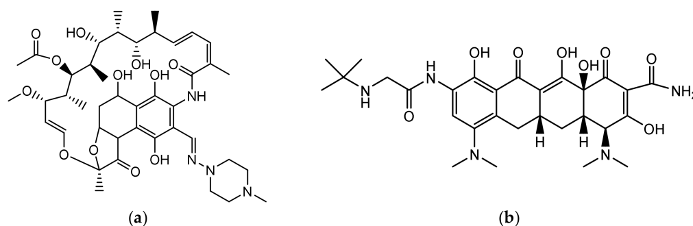
Scheme 1. Chemical structure of: (a) Rifampicin (RIFM): C_{43}H_{58}N_4O_{12} (822.94 g/mol), pK_{a1} = 1.7 and pK_{a2} = 7.9 [14]; (b) Tigecycline (TIGC): (585.65 g/mol), pK_a values: 2.8, 4.4, 7.4, 8.9, and 9.5 [15,16].
