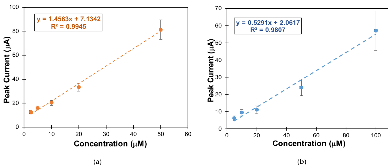
Figure 8. Calibration curves of SFX solutions in phosphate buffer solution, pH = 7.00 at 50 \text{mV}\cdot\text{s}^{-1} using (a) MWCNTs-CeO 2 @GCE, and (b) MWCNTs-Yb 2 O 3 @GCE sensors. Experimental conditions: counter electrode: Pt, reference electrode: Ag/AgCl; room temperature; stagnant solution, modified GCE sensor: 2 mg/mL MWCNTs and 0.5 mg/mL CeO 2 or Yb 2 O 3 and 10 \mu\text{L}/\text{mL} of 5% Nafion solution.
