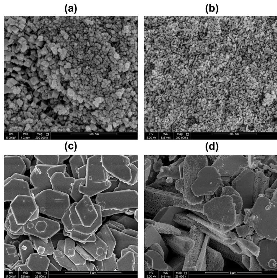
Figure 1. SEM images of CeO 2 (a,b) and Yb 2 O 3 (c,d) synthesized by hydrothermal method followed by annealing in absence (a,c) and in presence (b,d) of Triton TM X-100 as a surfactant.
