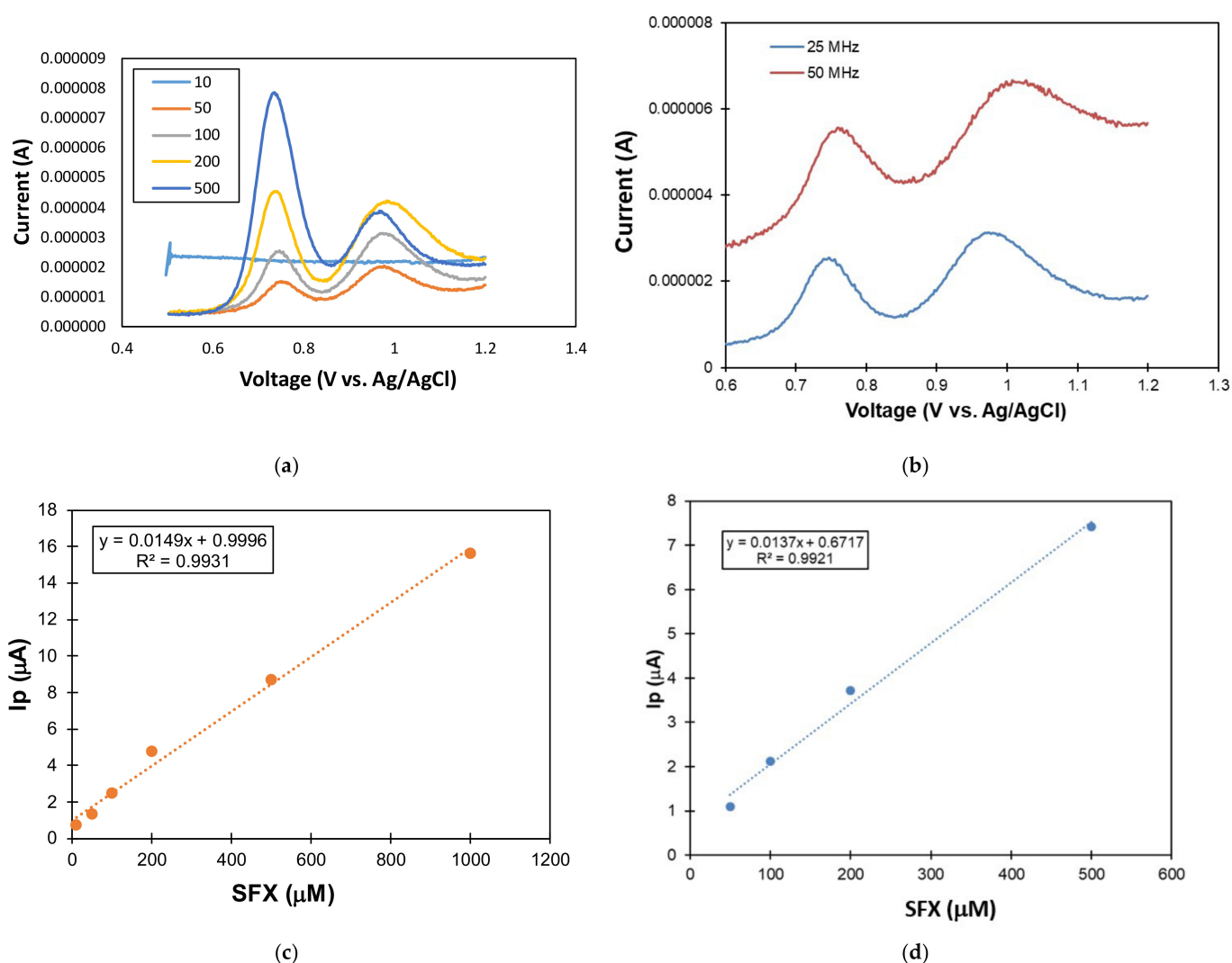
Figure 6. (a) Square wave voltammograms of SFX at 25 MHz at different concentrations (10–500 \mu\text{M} ), (b) Effect of the frequency on the voltammogram of 100 \mu\text{M} SFX. Calibration curves of SFX at: (c) 50 MHz and (d) at 25 MHz. Experimental conditions: working electrode: GCE (3 mm diameter), counter electrode: Pt wire, reference electrode: Ag/AgCl (3 M KCl), electrolyte: 0.05 M phosphate buffer (pH = 7.0), temperature: 25 ^{\circ}\text{C} , stagnant solution.
