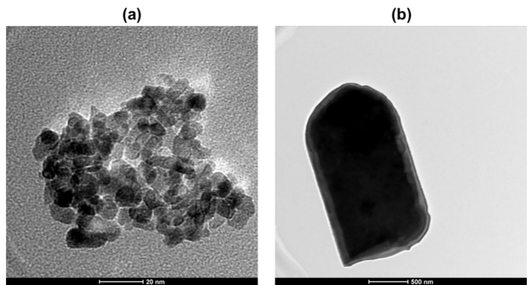
Figure 2. TEM images of (a) CeO 2 and (b) Yb 2 O 3 synthesized by hydrothermal method followed by annealing in presence of Triton TM X-100 surfactant.
