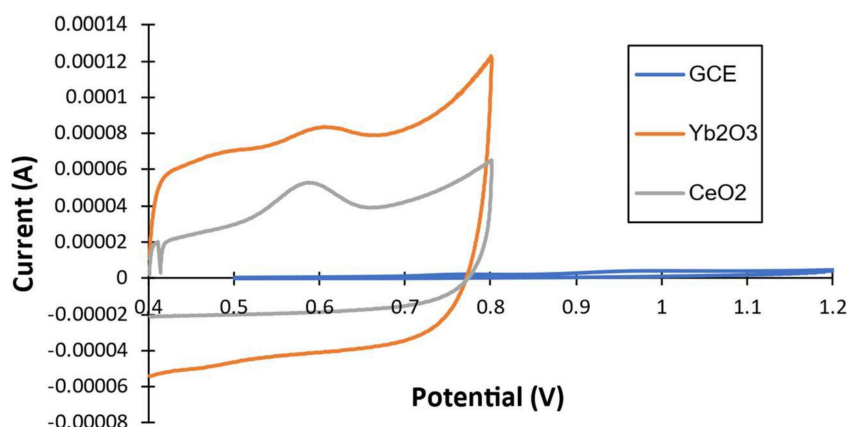
Figure 7. Voltammograms for electrochemical analysis of SFX using GCE electrode, MWCNTs-CeO 2 @GCE electrode and MWCNTs-Yb 2 O 3 @GCE electrode in phosphate buffer solution, pH = 7.0 at 50 \text{mV}\cdot\text{s}^{-1} for 20 \mu\text{M} . Experimental conditions: counter electrode: Pt, reference electrode: Ag/AgCl; room temperature; stagnant solution.
