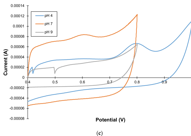
Figure 9. Anodic cyclic voltammograms of 100 \mu\text{M} SFX using (a) bare GCE, (b) MWCNTs-CeO 2 @GCE, and (c) MWCNTs-Yb 2 O 3 @GCE sensors in different buffer aqueous solutions (acetate: pH = 4.0, phosphate: pH = 7.0, and borate: pH = 9.0) at 50 \text{mV}\cdot\text{s}^{-1} . Experimental conditions: counter electrode: Pt, reference electrode: Ag/AgCl; room temperature; stagnant solution; modified GCE sensor: 2 mg/mL MWCNTs and 0.5 mg/mL CeO 2 or Yb 2 O 3 and 10 \mu\text{L}/\text{mL} of 5% Nafion solution.
