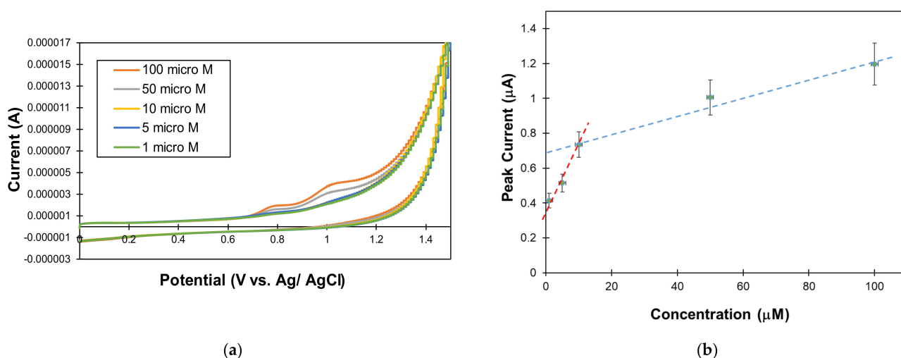
Figure 5. (a) Cyclic voltammograms and (b) Calibration curve of SFX solutions using GCE electrode in phosphate buffer solution, pH = 7.00 at 50 mV·s -1 . Experimental conditions: counter electrode: Pt, reference electrode: Ag/AgCl; room temperature; stagnant solution.
