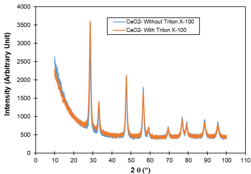
Figure 3. XRD spectra CeO 2 synthesized by hydrothermal method followed by annealing in absence and presence of Triton TM X-100 surfactant.
