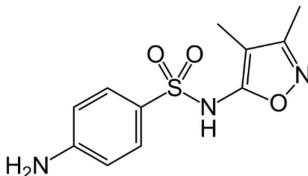
Scheme 1. Chemical structure of SFX. Chemical Formula: C_{11}H_{13}N_3O_3S (267.31 g/mol); IUPAC Name: 4-amino-N-(3,4-dimethyl-1,2-oxazol-5-yl)benzenesulfonamide; pK_{a1} : 1.5, pK_{a2} : 5.0 [12].
