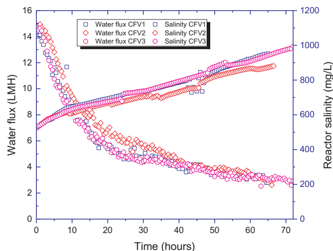
Fig. 3. Water flux profiles and salinity of mixed liquor in the OMBR system under three different cross-flow velocities of feed stream. Experiment conditions: DS = 35 g/L NaCl; FS = activated sludge mixed liquor; Temperature = 22 \pm 1 °C; AL – FS orientation. CFV 1 = 5.1 cm/s; CFV 2 = 8.5 cm/s; CFV 3 = 11.9 cm/s.
