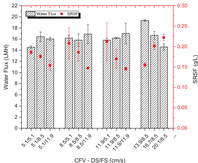
Fig. 2. Effects of different DS's cross-flow velocities on FO performance ( J_w and specific reverse solute flux - SRSF). Experiment conditions: DS = 35 g/L NaCl; FS = DI water; Temperature = 22 \pm 1 °C; AL - FS orientation.
