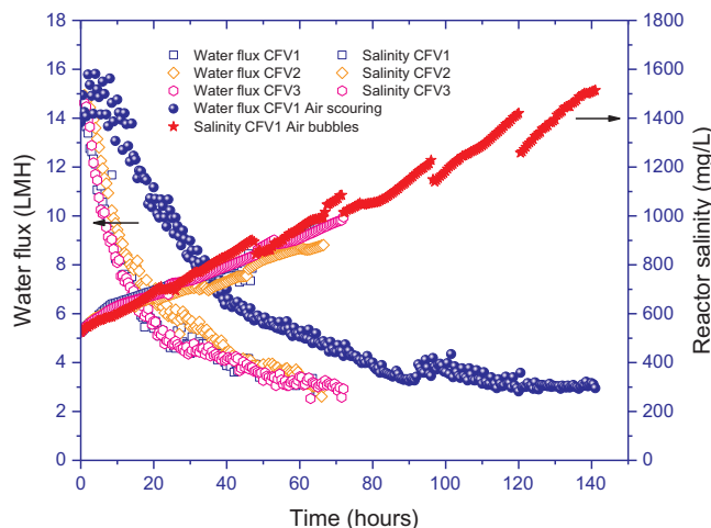
Fig. 4. Water flux profiles and salinity of mixed liquor in the OMBR system under the CFV 1 of feed stream with regular air scouring. Experiment conditions: DS = 35 g/L NaCl; FS = activated sludge mixed liquor; Temperature = 22 \pm 1 °C; AL – FS orientation.
