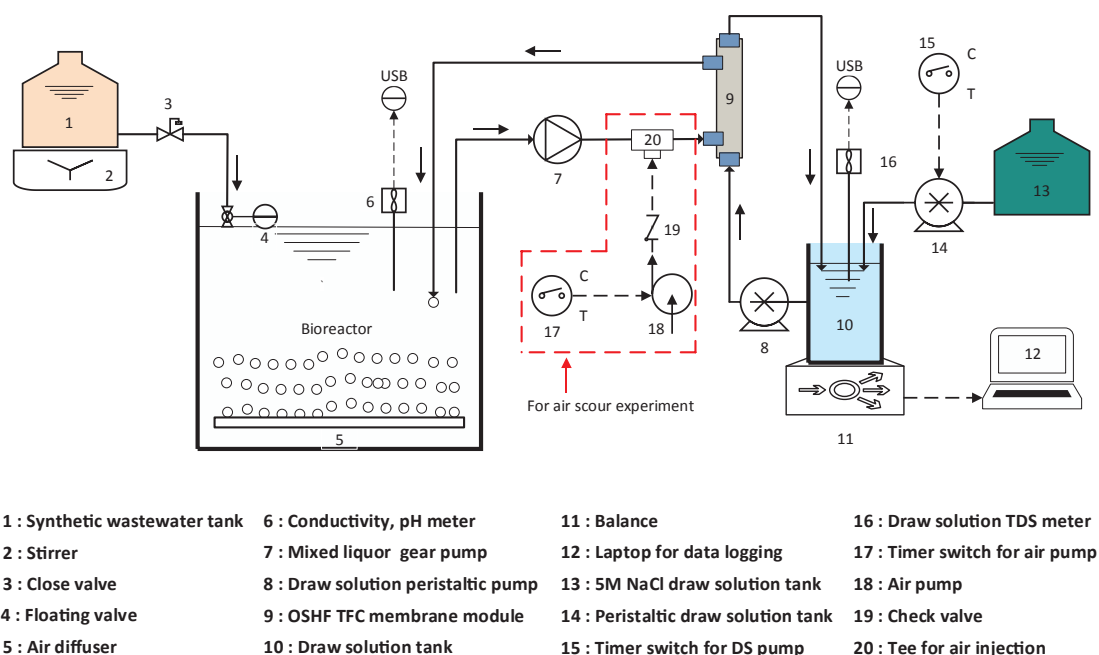
Fig. 1. Schematic diagram of side-stream osmotic membrane bioreactor system.
