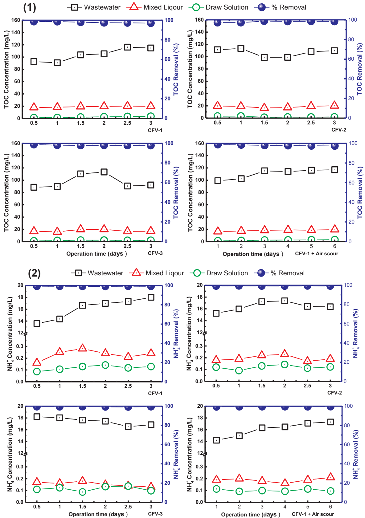
Fig. 5. Removal of pollutants of OMBR system operated under different cross flow velocities and with air scouring (1) TOC removal; (2) NH 4 + removal; (3) TN removal; and (4) PO 4 3- .
