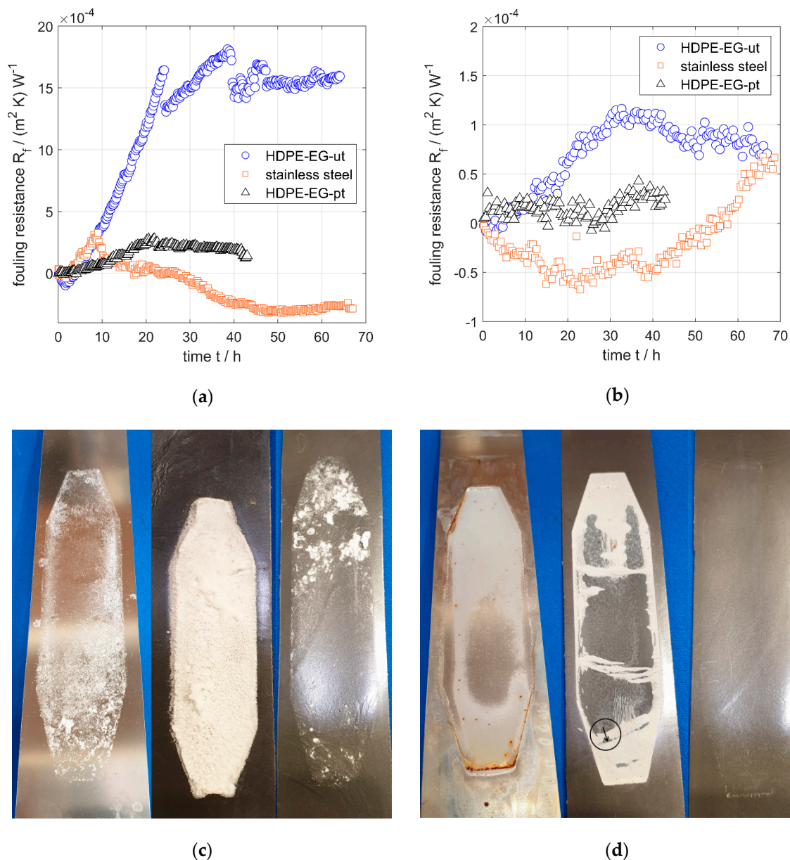
Figure 8. Measured fouling resistance due to crystallization fouling of (a) \text{CaSO}_4 , (b) mixed salts from seawater on the investigated heat transfer films. w = 45 \text{ g/kg} ; \dot{q} = 35 \text{ kW/m}^2 ; T_b = 30 \text{ }^\circ\text{C} ; \text{Resol} = 3100 , (c) scaling layer of \text{CaSO}_4 and (d) scaling layer caused by artificial seawater on stainless steel 1.4301 (left), HDPE-EG-ut (middle), HDPE-EG-pt (right).
