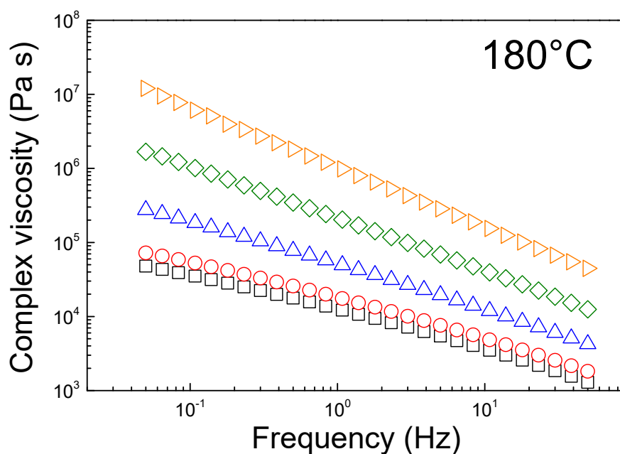
Figure 4. Dependence of complex viscosity on the frequency for various neat HDPE and various HDPE/EG composites at 180 °C, where □—neat HDPE, ○—90/10, △—70/30, ◇—50/50, ◀—30/70.
