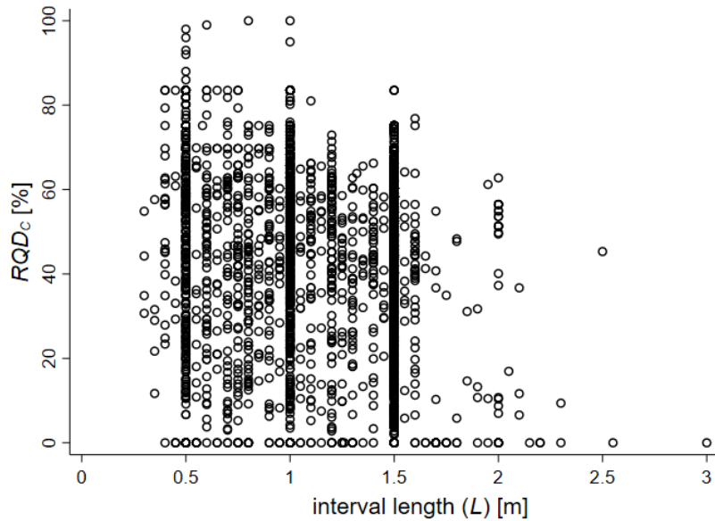
Fig. 5: RQD_C values against scanning interval lengths
