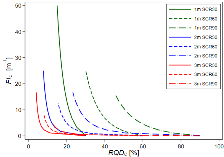
Fig. 4: Theoretical variation of FI_C versus RQD_C , for different scanning intervals and values of SCR for exponent a value (of RQD_C ) of 0.25
