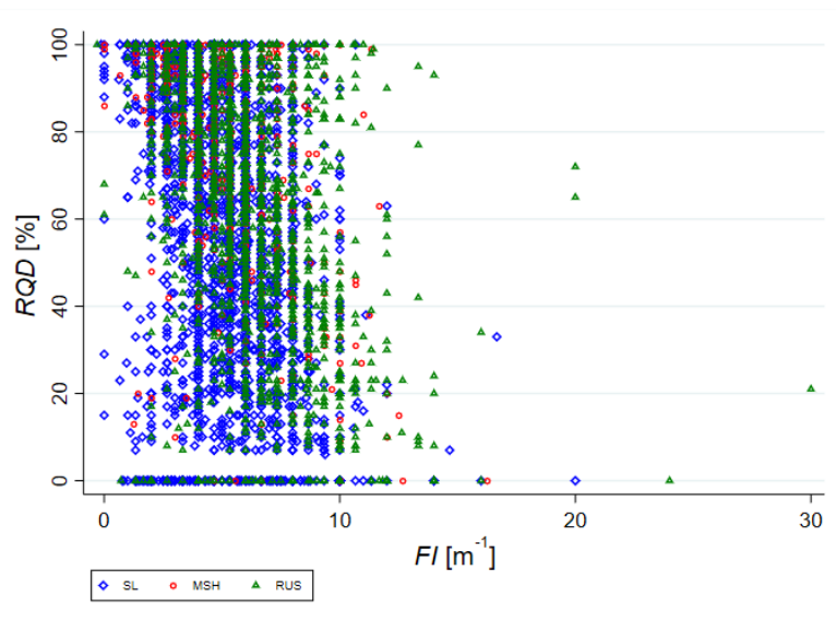
Fig. 2: Relation between RQD and frequency \lambda ( FI ) for Qatari rock masses
