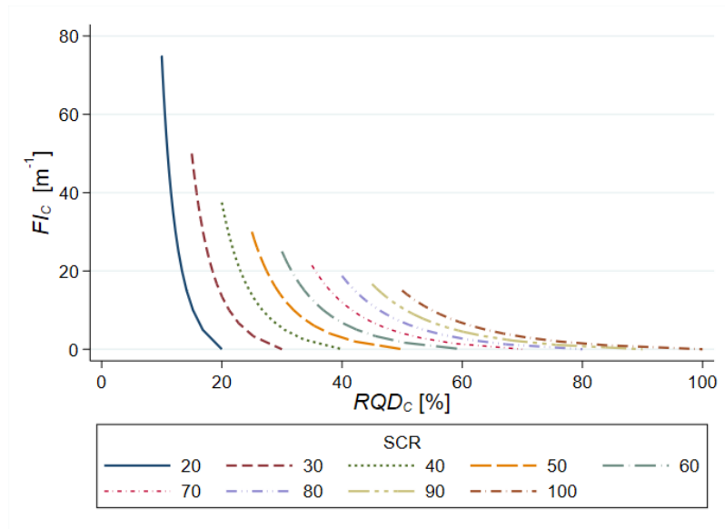
Fig. 3: Theoretical variation of FI_C versus RQD_C , for different values of SCR and exponent a value (of RQD_C ) of 0.25, and scanning interval of 1.0 m
