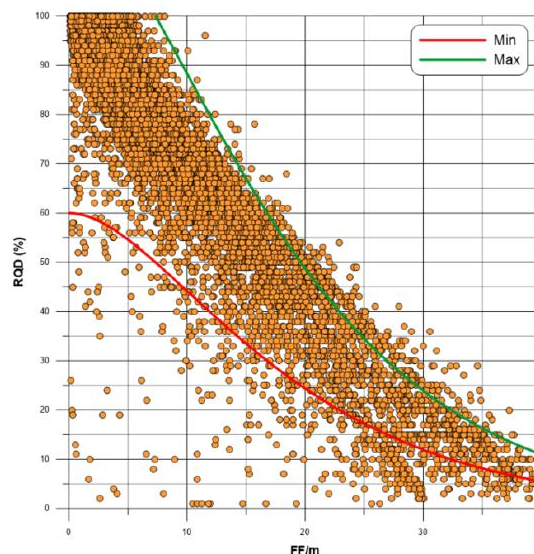
Fig. 1: Relation between RQD and mean fracture frequency \lambda ( FF – Fracture Frequency) according to Russo & Hormazabal (2019)
