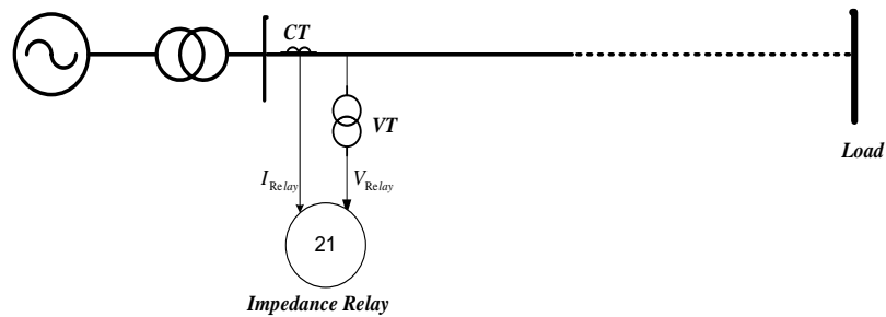
Fig.43: Principles and location of the impedance relay
