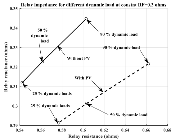
Fig.11: Relay impedance with different dynamic load percentage and constant R_F with and without PV
