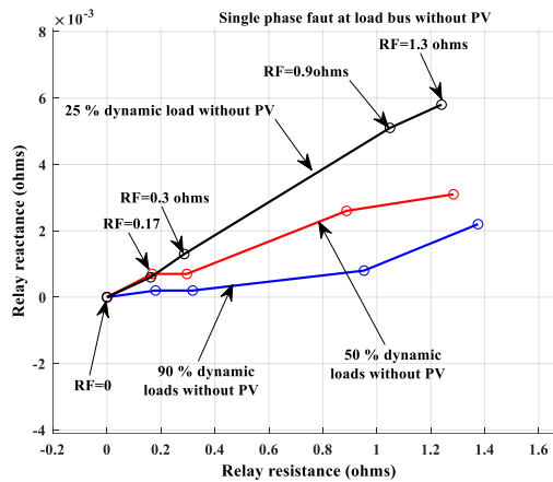
Fig.155: Single line to ground fault at load bus for different dynamic load percentage without PV
