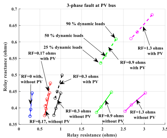
Fig.154: Relay impedance for 3-line to ground fault at PV bus (bus 3) for constant R_f
