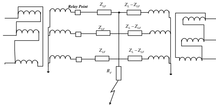
Fig.78.a: Single line to ground fault with fault resistance
