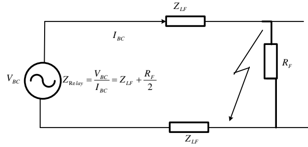
Fig.65.b: line to line short circuit considering R_F
