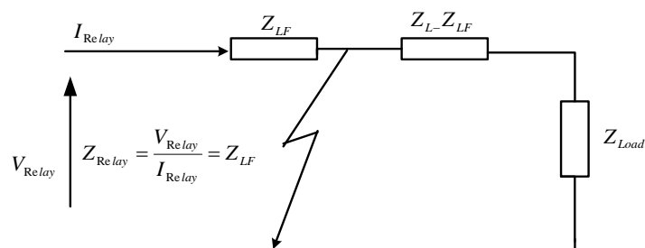
Fig.54.b: Protective impedance relay during fault
