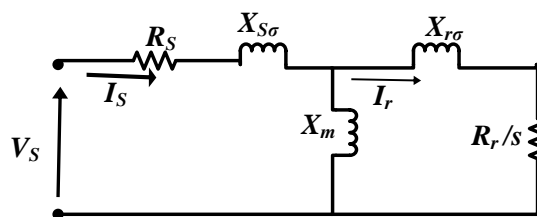
Fig.32: Equivalent circuit referred to stator of the asynchronous machine
