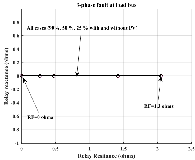
Fig.199: Relay impedance for 3-phase fault at load bus (all cases)
