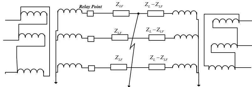
Fig.67: Solid ground single line to ground fault ( R_f = 0 )
