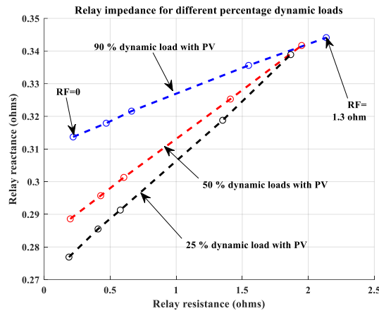
Fig.910: Relay resistance and reactance for different dynamic load percentages with PV
