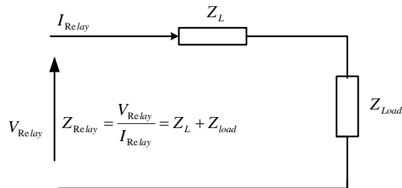
Fig.54.a: Protective impedance relay during normal conditions
