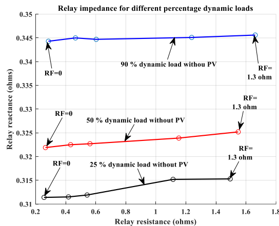
Fig.98: Relay impedance at different dynamic load percentages without PV
