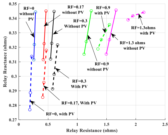
Fig.1212: Relay impedance with different dynamic load percentages and different R_F ( R_F = 0 to R_F = 1.3 ohm) with and without PV for SLG fault at PV bus (bus3).
