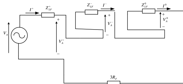
Fig.78.b: Equivalent circuit of single line to ground fault considering fault resistance
