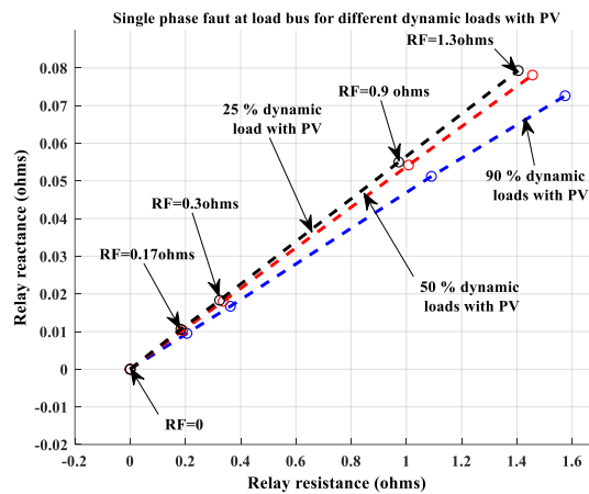
Fig.1616: Single line to ground fault at load bus for different dynamic loads with PV
