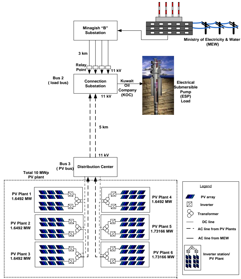
Fig.21.b: Case study, power system configuration and single line diagram (Abdullah et al., 2016)[18]
