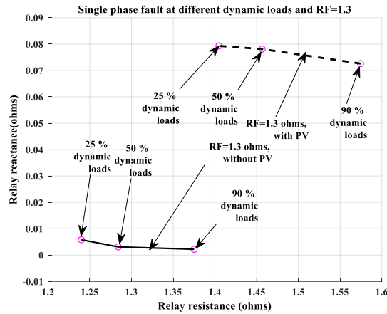
Fig.1818: Single line to ground fault at load bus with different percentages of dynamic loads, and constant R_F ( R_F = 1.3 \Omega ), with and without PV.
