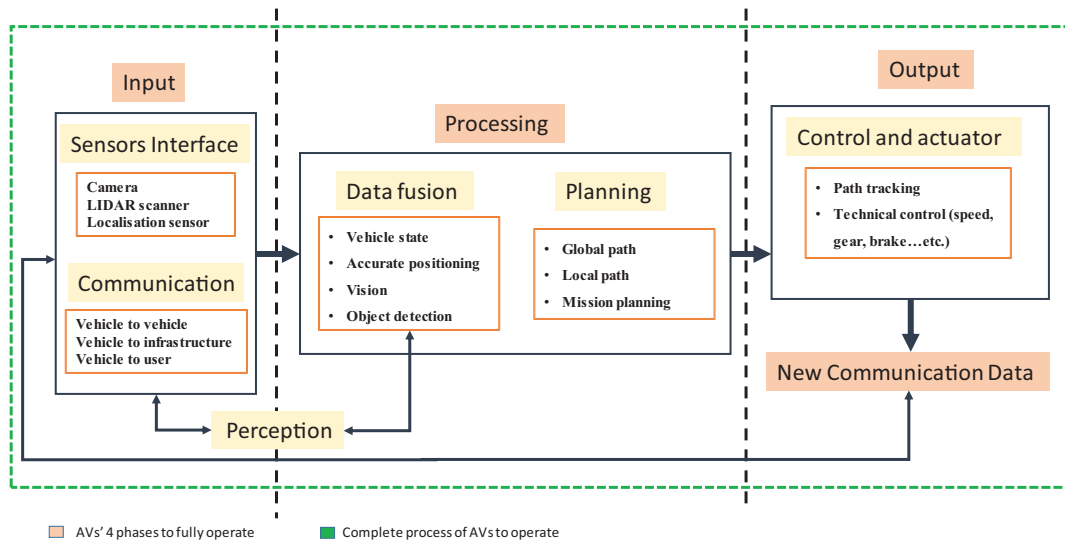
Fig. 11. Connected autonomous vehicle system architecture overview, reproduced from [113,124,128].
