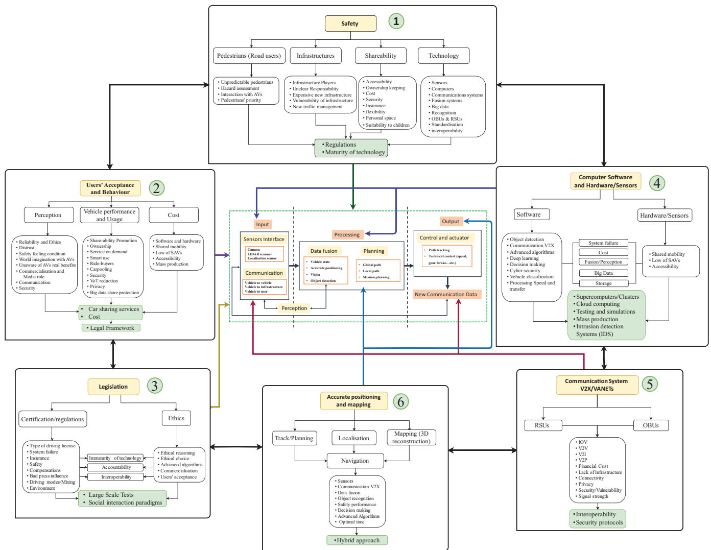
Fig. 14. Framework assembling all the barriers and their factors combined with AVs system architecture.
