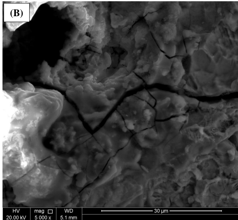
Figure 13[A and B]. SEM images illustrate the formation of pits which acted as active site for initiation of chloride stress cracking corrosion on the outer surface of 316L stainless steel.
