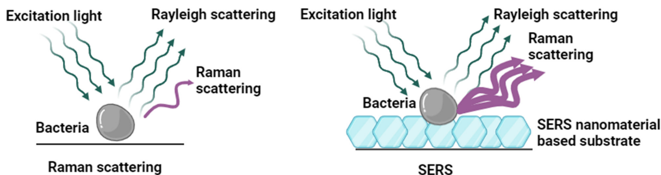
Figure 1. The comparison of normal Raman scattering and SERS scattering. ( Left panel ), Raman scattering of bacteria without surface enhancement. ( Right panel ), SERS enhancement by nanomaterials. Created with BioRender.com (accessed on 19 July 2024).
