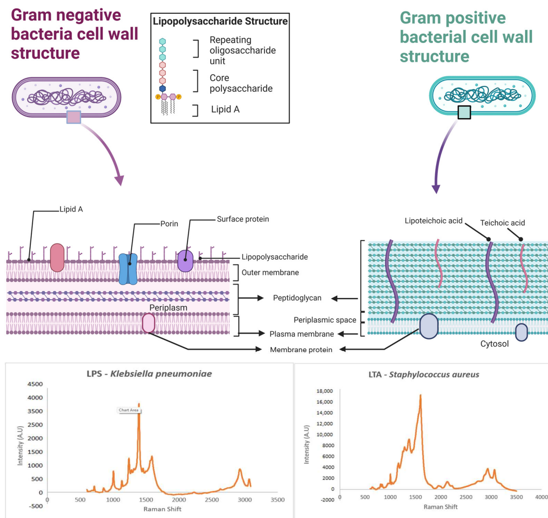
Figure 4. The cellular structure differences between Gram-positive and Gram-negative bacteria, SERS spectra of Gram-negative lipopolysaccharide and Gram-positive lipoteichoic acid. Created with BioRender.com (accessed on 19 July 2024).
