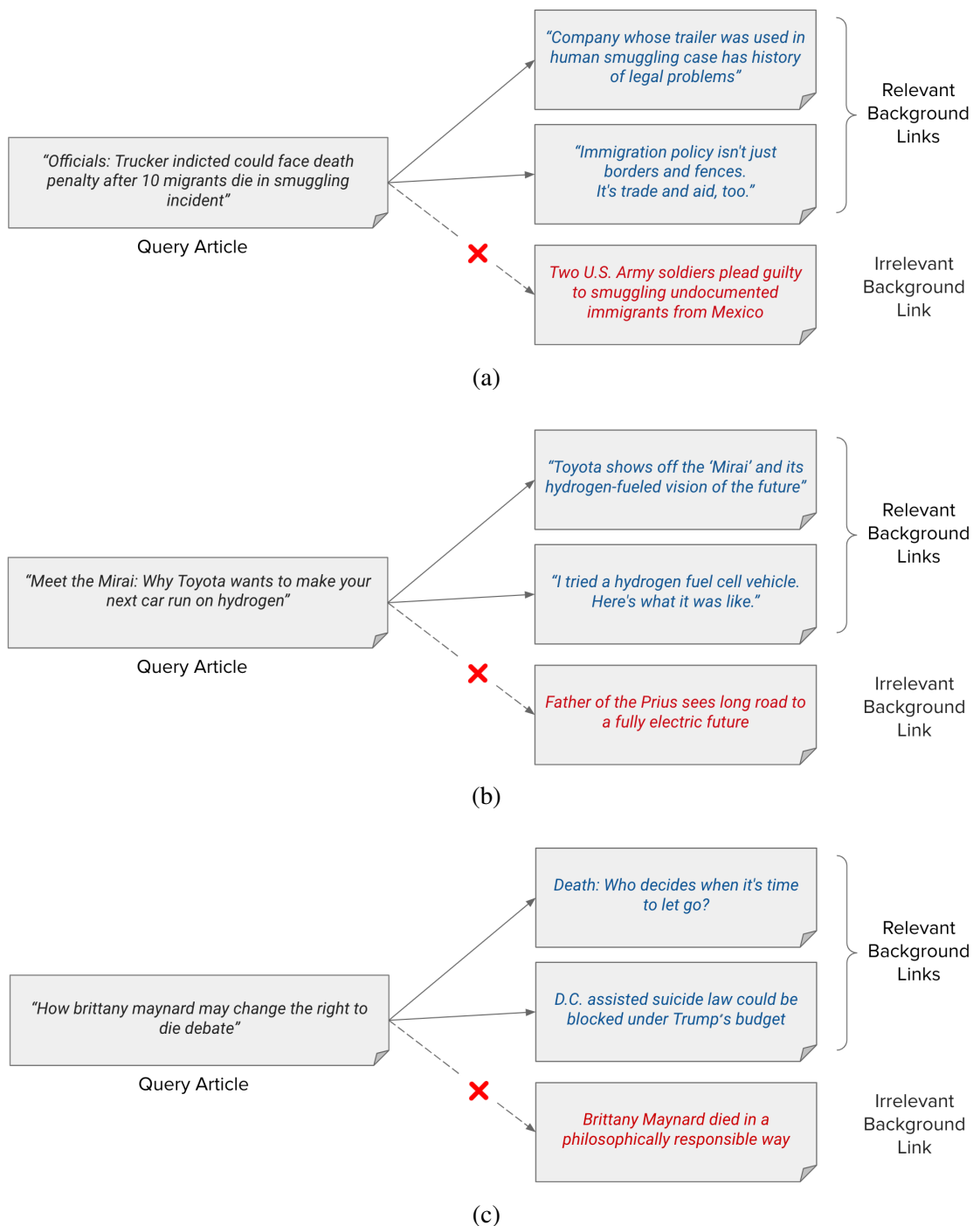
Figure 1.4. Examples of news background linking drawn from the TREC dataset for the news track
