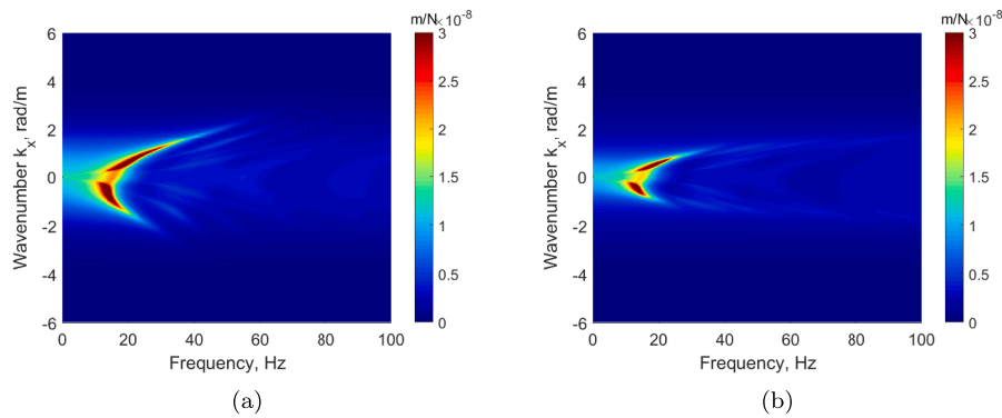
Fig. 9. Contour plots of the rail point receptance in the frequency-wavenumber domain for tracks on ground Type G1 due to moving harmonic loads at v = 33.3 m/s with respect to wavenumber k_x . (a) Ballasted track Case B1; (b) slab track Case S1.
