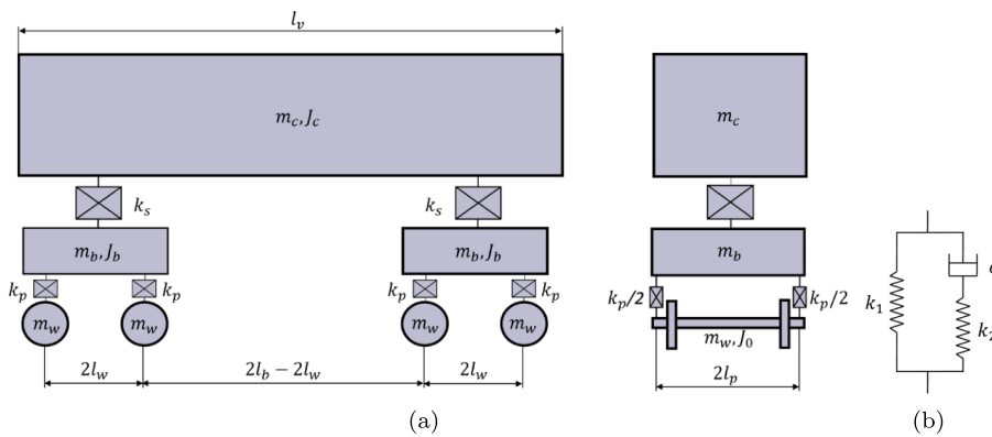
Fig. 1. (a) Vehicle model with primary and secondary suspensions. (b) Suspension model.
