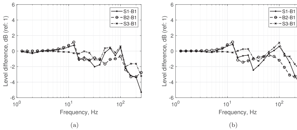
Fig. 18. One-third octave level differences, relative to ballasted track B1, of slab track S1, ballasted track B2 and slab track S3; all for ground Type G1 at 8 m from the track centreline for train speed: (a) 33.3 m/s and (b) 83.3 m/s.
