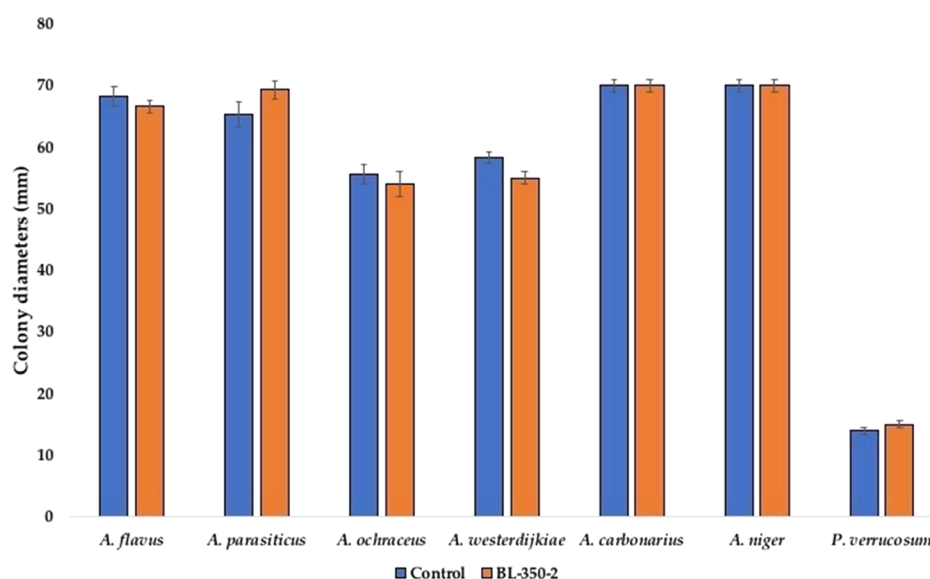
Figure 3. Colony diameters of B. licheniformis (BL350-2) exposed fungi on fresh PDA media vs never exposed fungi (control) fungi. Mycelial plugs were removed from the margins of fungal colonies, transferred to fresh PDA, and incubated for 10 days for the measurement of colony diameters (mm). Bars represent the means of nine observations \pm SD.
