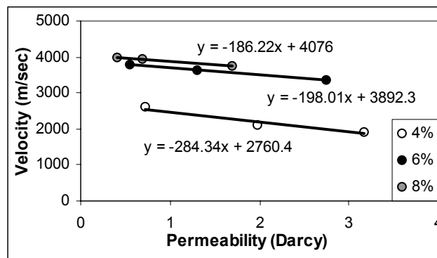
Fig. (7) Rock permeability versus sonic velocity at varying cementation ratios.
