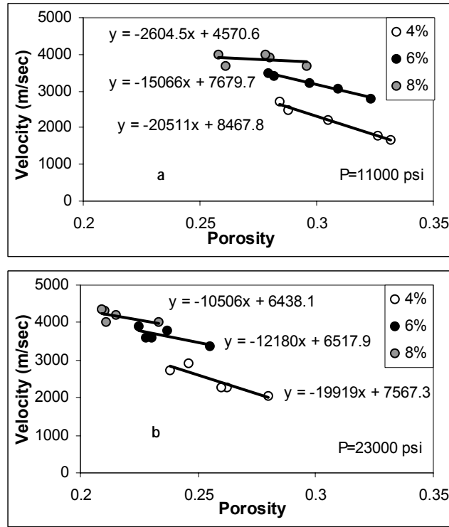
Fig. (4a-b) Rock porosity versus sonic velocity at varying cementation and compaction.
