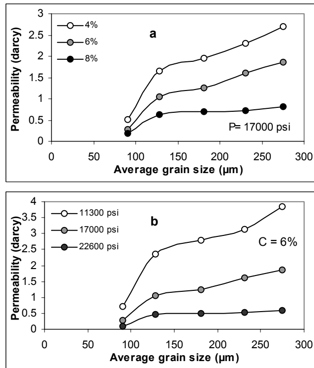
Fig. (3a-b) Effect of grain size on rock permeability (Ref. 8)
