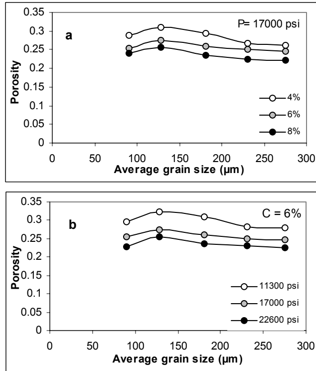
Fig. (2a-b) Effect of grain size on rock porosity
