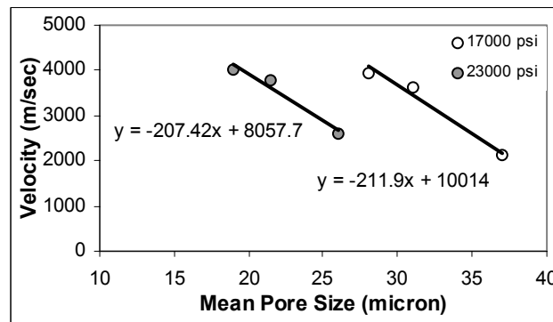
Fig. (6) Mean pore size versus sonic velocity at varying compaction
