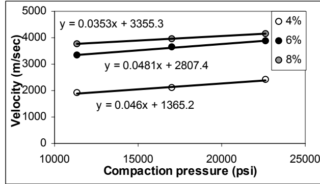
Fig. (5) Compaction pressure versus sonic velocity at varying cementation.
