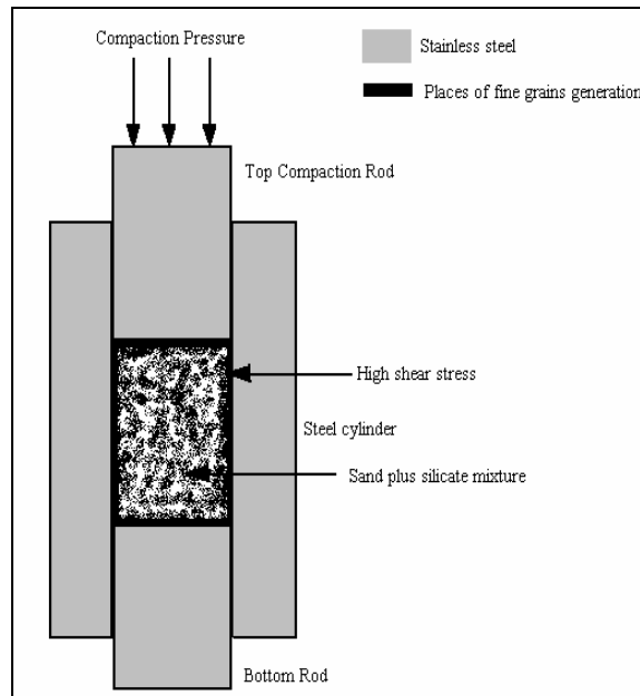
Fig. (1a) Compaction Cell
