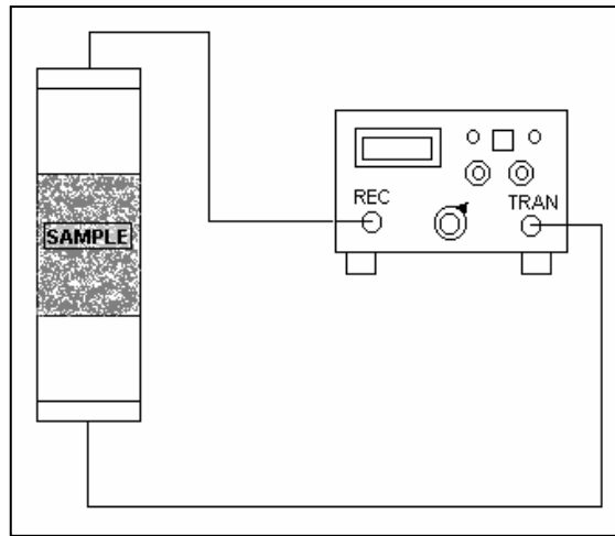
Fig. (1b) PUNDIT connected to the rock sample.
