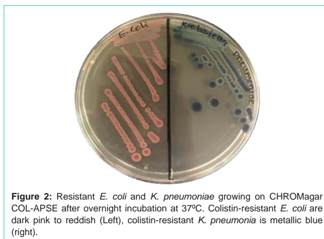
Figure 2: Resistant E. coli and K. pneumoniae growing on CHROMagar COL-APSE after overnight incubation at 37°C. Colistin-resistant E. coli are dark pink to reddish (Left), colistin-resistant K. pneumoniae is metallic blue (right).
