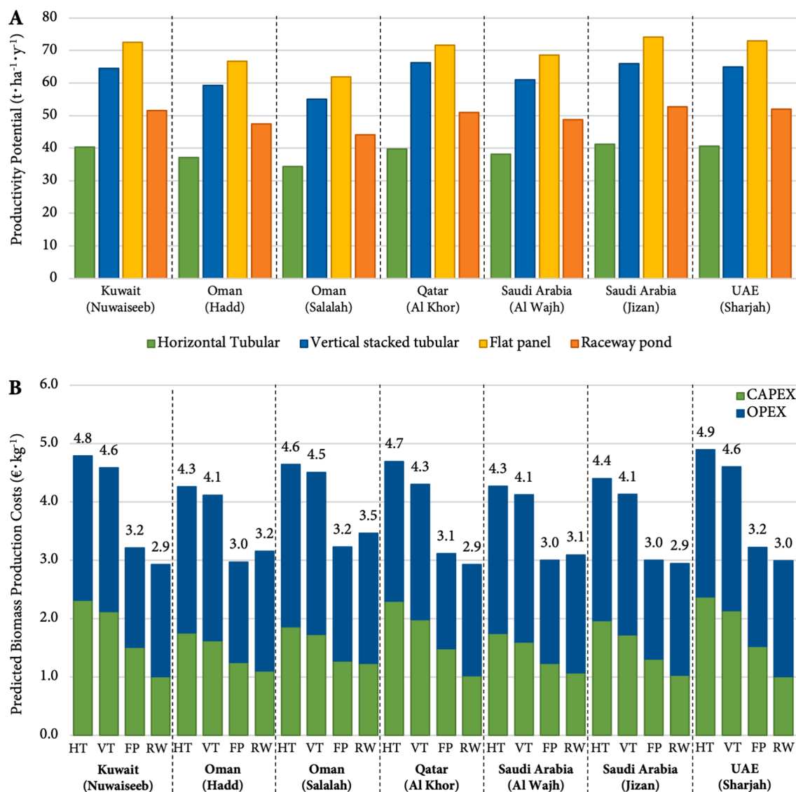
Fig. 1. Projected biomass productivities in t·ha -1 ·y -1 (A) and biomass production costs for both CAPEX and OPEX in €·kg -1 (B), for 100 ha facility in different GCC locations, and four bioreactor types (HT: Horizontal tubular, VT: Vertical stacked tubular, FP: Flat panel, RW: Raceway pond).
