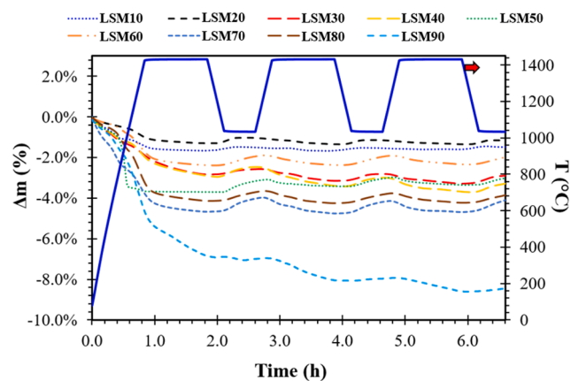
Fig. 10. LSM perovskites: TGA profiles obtained during three cycles (TR at 1400 °C for 60 min, CS at 1000 °C for 30 min, and heating/cooling rate = 25 °C/min).
