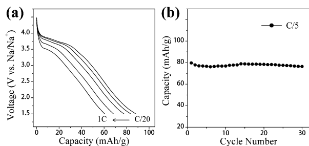
Figure 3. (a) The rate capability of \text{Na}_2\text{MnP}_2\text{O}_7 at various C-rates during discharge and (b) discharge cycle life of \text{Na}_2\text{MnP}_2\text{O}_7 , measured at C/5. In (a), the discharge rates are C/20, C/10, C/5, C/2, 1C from right to left.
