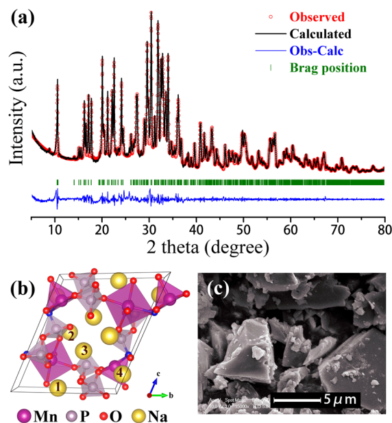
Figure 1. (a) The XRD spectrum and whole pattern fitting of \text{Na}_2\text{MnP}_2\text{O}_7 ( R_p = 3.18 , R_{wp} = 4.59 , \chi^2 = 2.35 ). (b) The crystal structure of the triclinic \text{Na}_2\text{MnP}_2\text{O}_7 where the purple, gray, red, and yellow spheres represent Mn, P, O, and Na atoms, respectively. The four sodium sites, Na1 – Na4 are also denoted. In this periodic image, the octahedral \text{MnO}_6 and pyramidal \text{MnO}_5 moieties share one oxygen atom (blue) to make \text{Mn}_2\text{O}_{10} unit. (c) An SEM image of the as-synthesized sample shows particle sizes in the range of 2–7 \mu\text{m} .
