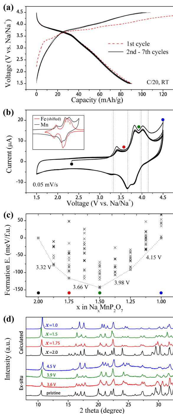
Figure 2. (a) The galvanostatic charge–discharge curves and (b) CV profiles of \text{Na}_2\text{MnP}_2\text{O}_7 measured at room temperature. The CV profiles of \text{Na}_2\text{FeP}_2\text{O}_7 12 in the inset of (b) are shifted by 0.85 V for clear comparison. The four dotted lines correspond to the calculated voltages as shown in (c). (c) Calculated formation energies at various compositions and a convex hull for potential calculations. (d) The ex-situ XRD patterns obtained at the potentials marked in (b) together with the simulated patterns at the corresponding compositions marked in (c).
