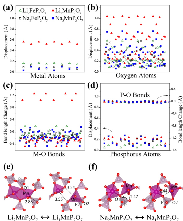
Figure 4. Displacements of (a) TMs and (b) oxygen-atoms, and (c) M-O bond length changes for A_2MP_2O_7 ( A = \text{Li} and \text{Na} , M = \text{Fe} and \text{Mn} ) during full charging. The x -axes in (a-c) correspond to the different crystallographic sites of the relevant elements. (d) The displacements of phosphorus atoms (left) and P-O bond length changes (right). For the different samples, the same color codes are used for (b-d) as in (a). The rearrangements of atomic positions and their bond lengths between the charged and discharged states for (e) \text{Li}_2\text{MnP}_2\text{O}_7 and (f) \text{Na}_2\text{MnP}_2\text{O}_7 . Atomic colors are the same as in Figure 1a and the numbers are M-O distances in Å.
