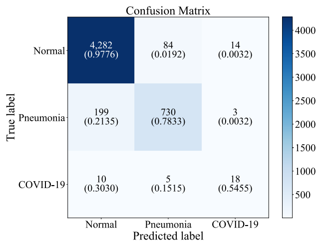
(a) Proposed CNN without data augmentation.
