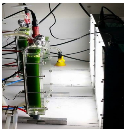
Figure 1. 1 L flat panel airlift type PBR with full control of culture conditions (i.e., constant or fluctuation regimes of light and/or temperature).
