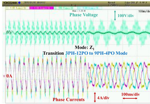
FIGURE 10 Experimental voltage and currents of PPMIM drive during transient mode Z_1 shown in Figure 6
