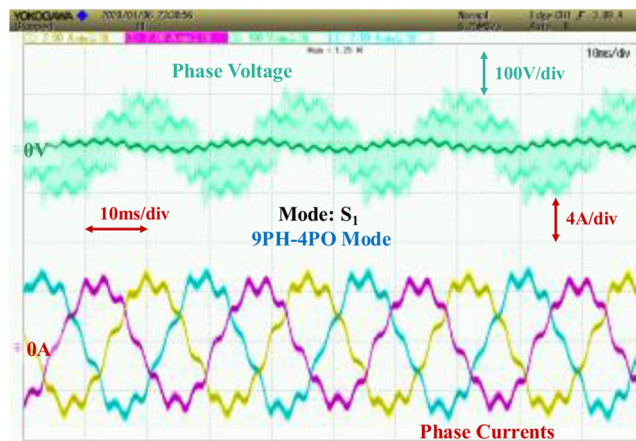
FIGURE 11 Steady-state voltage and currents of PPMIM drive in 9PH-4PO mode ( S_1 ) with IFOC
