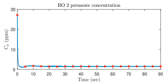
Fig. 10. RO pass 2 permeate concentration.
