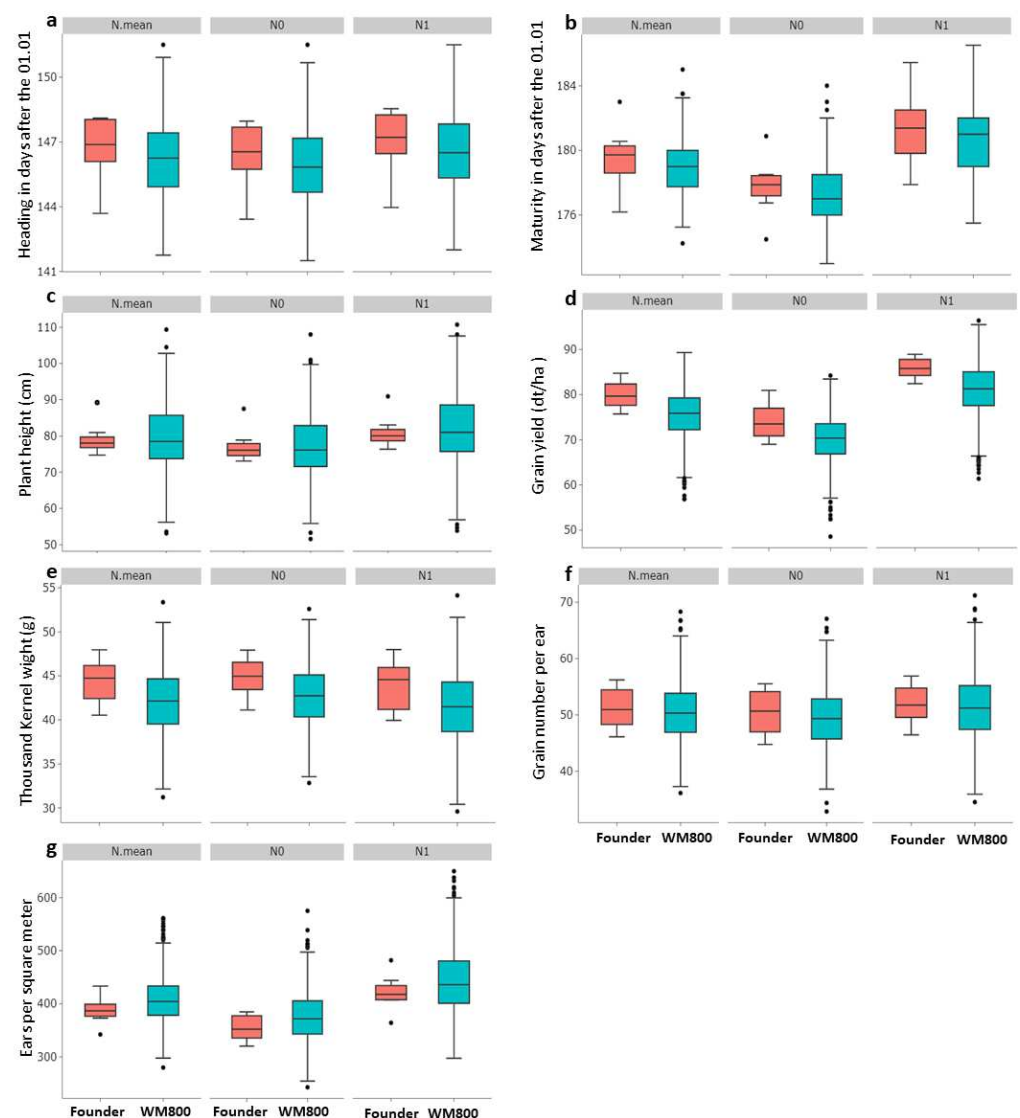
Figure 1. Box-Whisker-Plots indicating variations among WM-800 lines and founders across (N.mean) and within N treatments (N0 and N1) for seven traits studied (subplots (a–g)). For all traits, the ANOVA indicated highly significant differences between N treatments at p < 0.001 or p < 0.01 for both population WM-800 and the founders.
