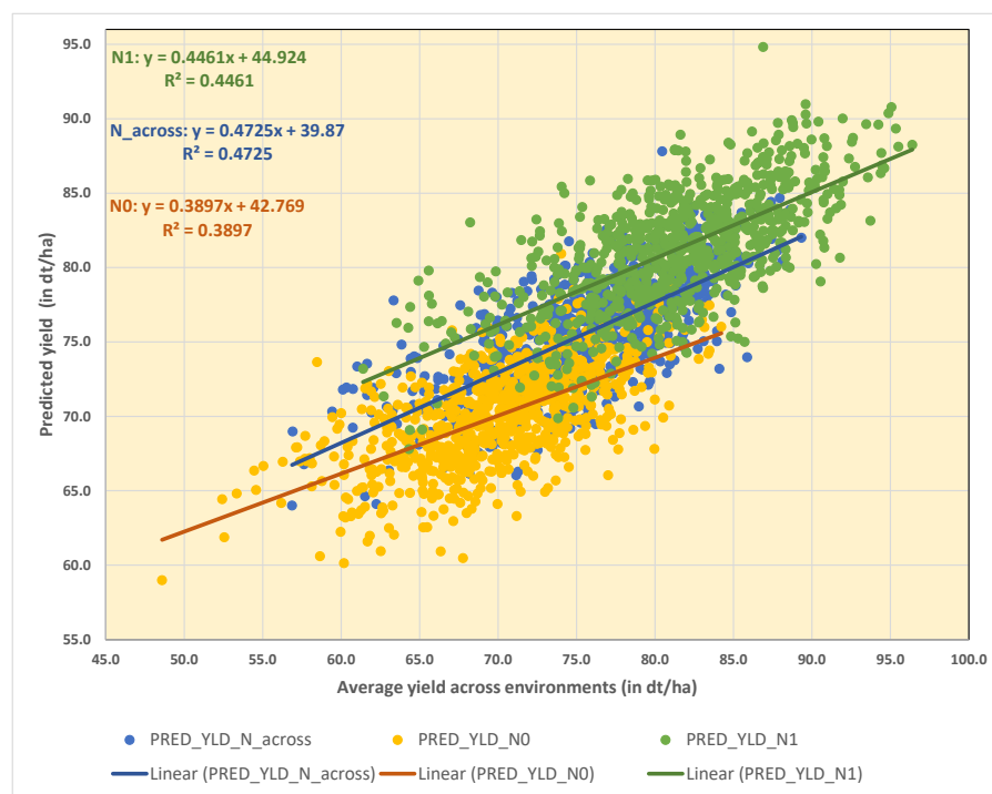
Figure 4. Multiple linear regression plot of predicted yield by actual yield averaged across N treatments and within N0 and N1 environments, respectively. The stepwise regression procedure HPREG selected 9–10 informative QTL alleles and 3 informative quantitative traits for yield prediction.
