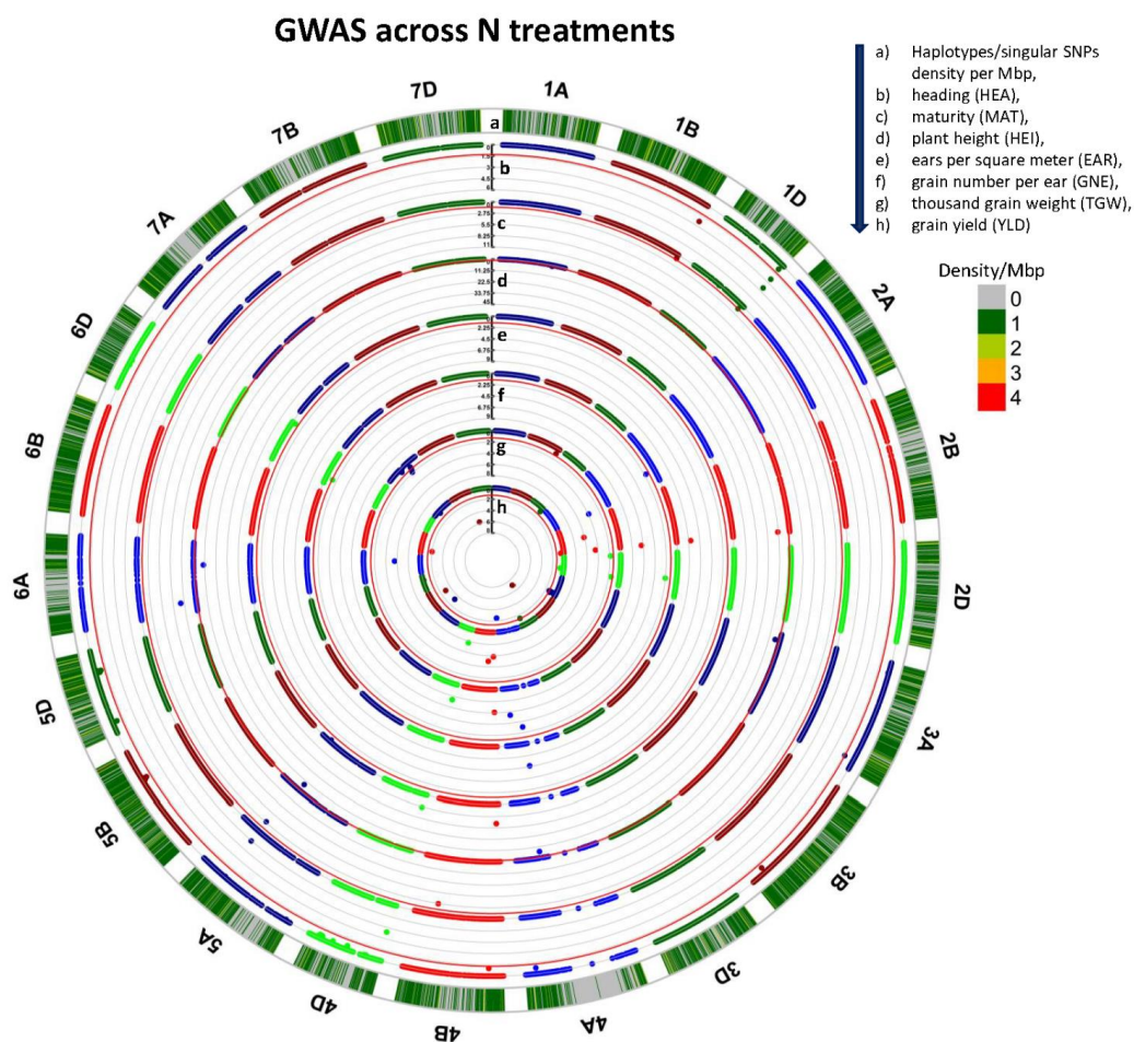
Figure 3. Circular Manhattan plots of genome-wide association scan for seven traits studied in WM-800 across N treatments.
