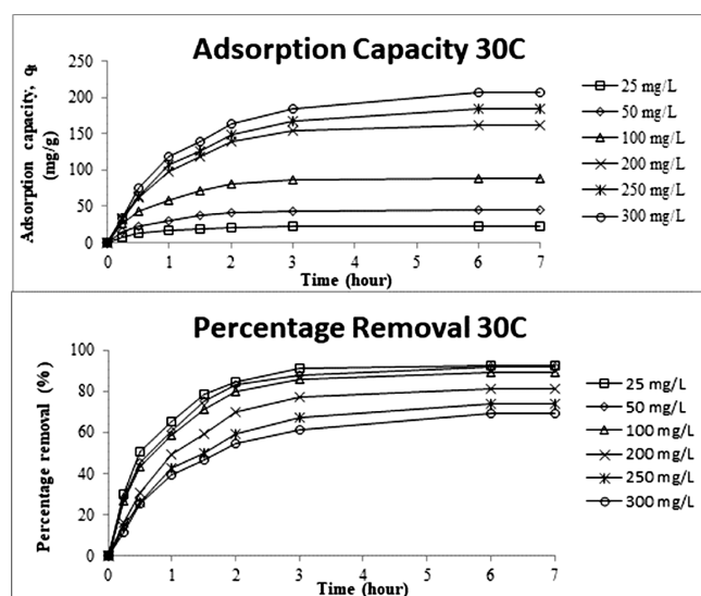
Figure 5. Plots of (a) adsorption capacity and (b) percentage removal of RBBR onto LSDAC versus time at 30 °C for different initial concentrations of RBBR (original pH of RBBR, 0.2 g adsorbent dosage, and 200 mL of solution).
