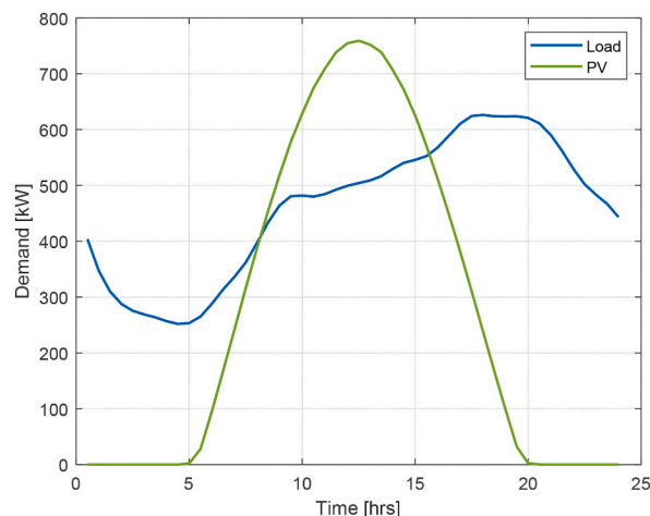
Fig. 4. Exact power of load and PV for 24 h.
